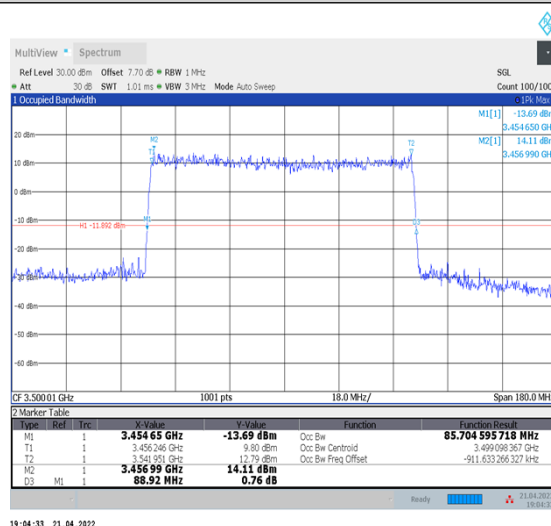
1-N78-3450-3550--30-90-M-4-DFT-64QAM-Outer_Full-240@0-Ant1-85.705-88.920-≤90-PASS
