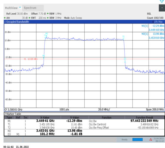
1-N78-3450-3550--30-100-L-6-CP-QPSK- Outer_Full-273@0-Ant1-97.443-101.200-≤100-PASS
