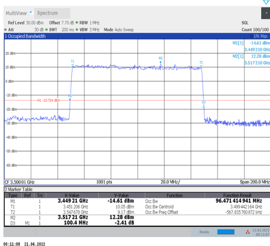
1-N78-3450-3550--30-100-L-5-DFT-256QAM- Outer_Full-270@0-Ant1-96.471-100.400-≤100-PASS
