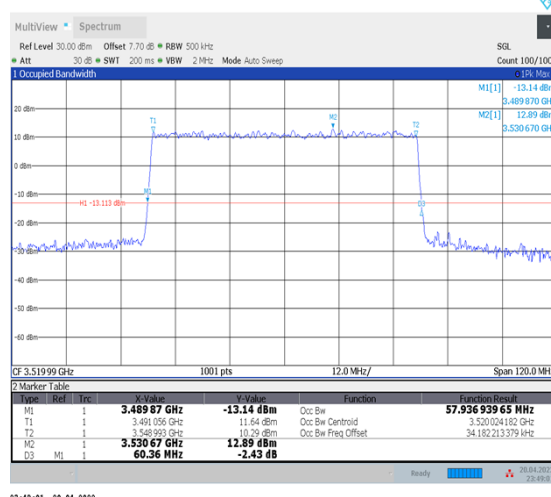
1-N78-3450-3550--30-60-H-4-DFT-64QAM-Outer_Full-162@0-Ant1-57.937-60.360-≤60-PASS
