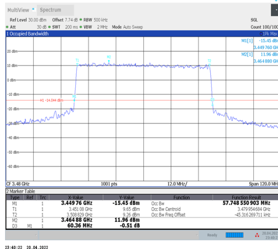
1-N78-3450-3550--30-60-L-8-CP-64QAM- Outer_Full-162@0-Ant1-57.749-60.360-≤60-PASS
