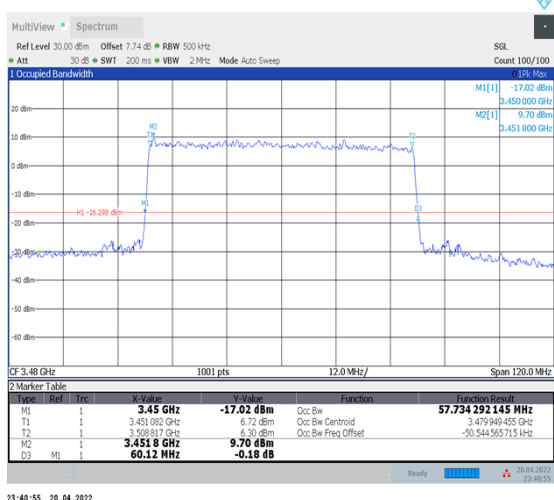
1-N78-3450-3550--30-60-L-9-CP-256QAM- Outer_Full-162@0-Ant1-57.734-60.120-≤60-PASS
