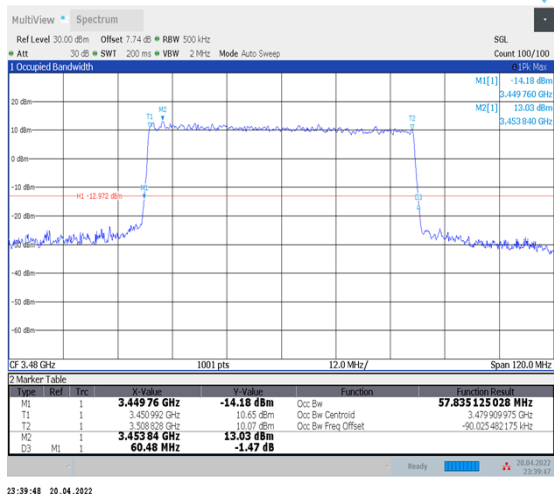
1-N78-3450-3550--30-60-L-7-CP-16QAM- Outer_Full-162@0-Ant1-57.835-60.480-≤60-PASS
