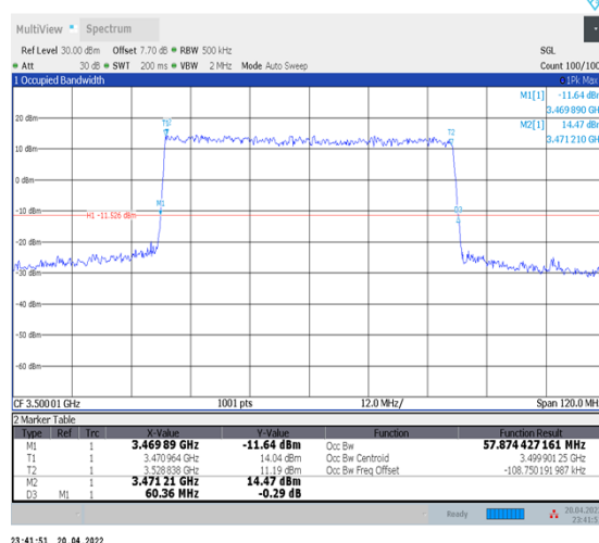
1-N78-3450-3550--30-60-M-1-DFT-QPSK- Outer_Full-162@0-Ant1-57.874-60.360-≤60-PASS
