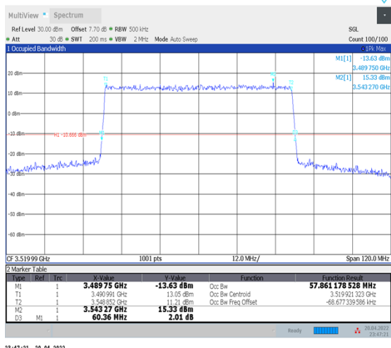
1-N78-3450-3550--30-60-H-1-DFT-QPSK-Outer_Full-162@0-Ant1-57.861-60.360-≤60-PASS
