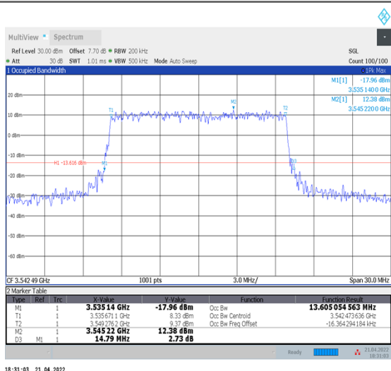
1-N78-3450-3550--30-15-H-6-CP-QPSK-Outer_Full-38@0-Ant1-13.605-14.790-≤15-PASS
