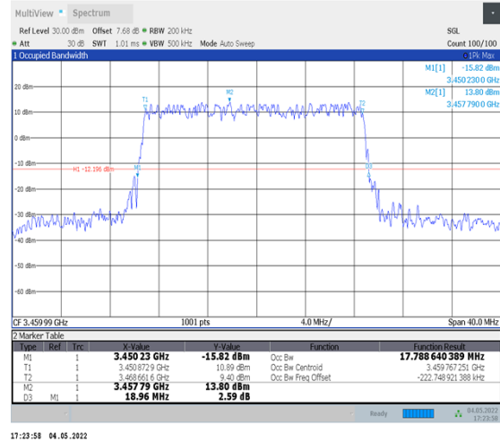
1-N78-3450-3550--30-20-L-4-DFT-64QAM-Outer_Full-50@0-Ant1-17.789-18.960-≤20-PASS
