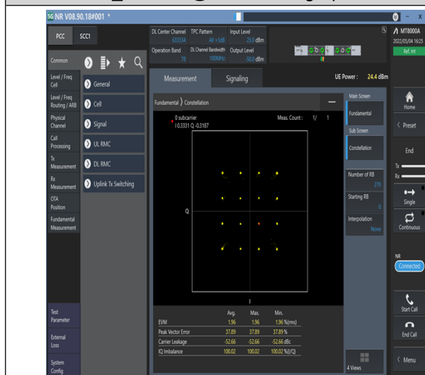
1-N78-3450-3550--30-100-M-3-DFT-16QAM- Outer_Full-270@0-Ant1-see graph-PASS
