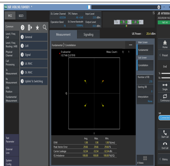
1-N78-3450-3550--30-100-M-2-DFT-QPSK- Outer_Full-270@0-Ant1-see graph-PASS
