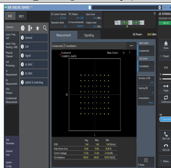
1-N78-3450-3550--30-100-M-4-DFT-64QAM- Outer_Full-270@0-Ant1-see graph-PASS
