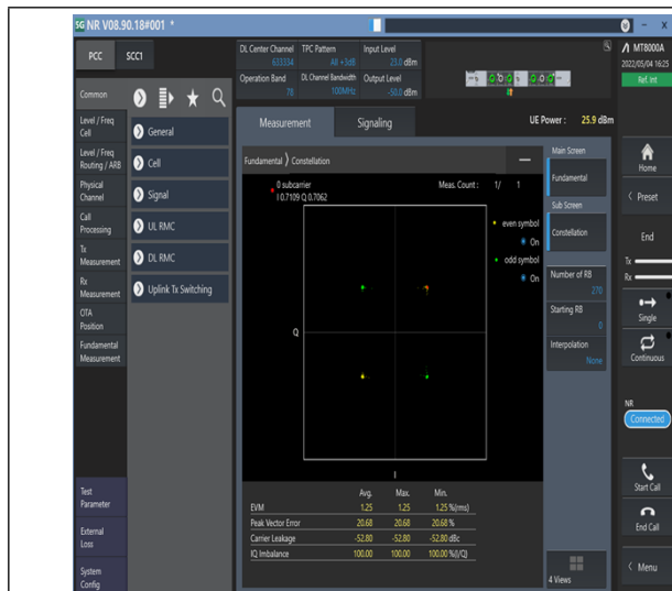
1-N78-3450-3550--30-100-M-1-DFT-PI2BPSK- Outer_Full-270@0-Ant1-see graph-PASS
