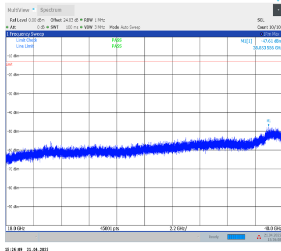
1-N77-3700-3980--30-100-L-1-DFT-PI2BPSK- Inner_1RB_Left-1@1-18000-40000-Ant1--47.61--13- PASS
