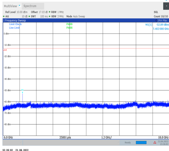
1-N77-3700-3980--30-100-L-1-DFT-PI2BPSK- Inner_1RB_Left-1@1-6000-18000-Ant1--52.89--13- PASS
