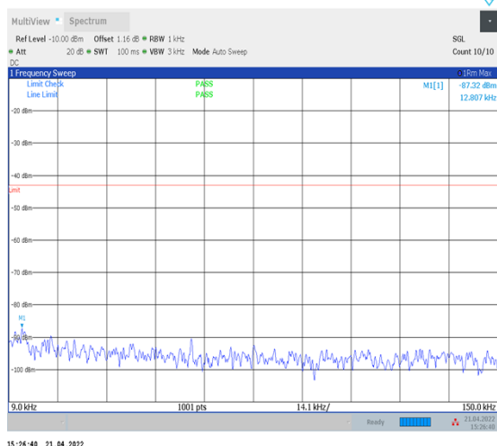
1-N77-3700-3980--30-100-M-1-DFT-PI2BPSK- Inner_1RB_Left-1@1-0.009-0.15-Ant1--87.32--43- PASS
