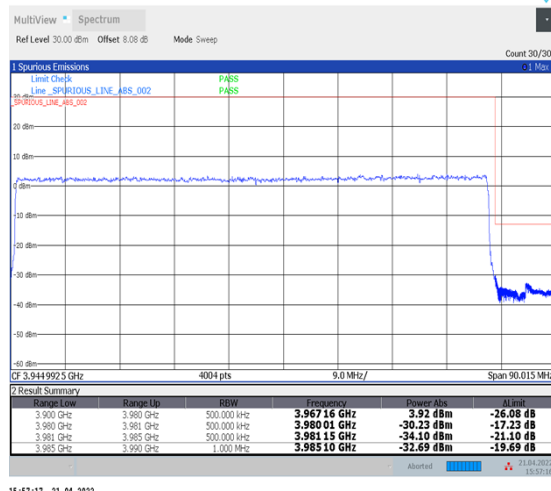
1-N77-3700-3980--30-80-H-3-DFT-PI2BPSK-Outer_Full-216@0-Ant1-PASS-see graph
