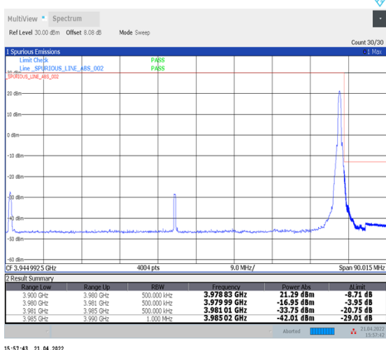
1-N77-3700-3980--30-80-H-5-CP-QPSK-Edge_1RB_Right-1@216-Ant1-PASS-see graph
