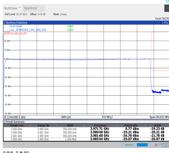
1-N77-3700-3980--30-80-H-6-CP-QPSK-Outer_Full-217@0-Ant1-PASS-see graph
