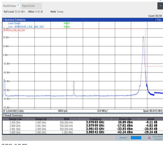
1-N77-3700-3980--30-80-H-2-DFT-PI2BPSK-Edge_1RB_Right-1@216-Ant1-PASS-see graph
