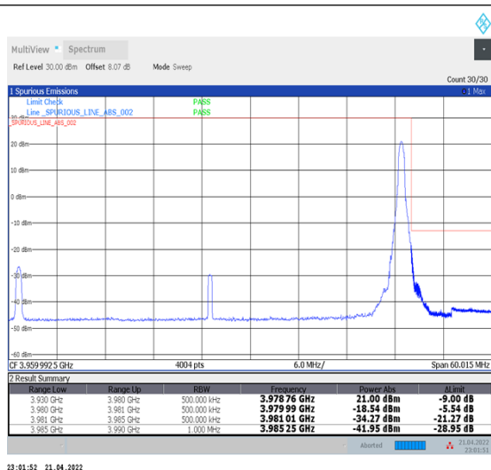
1-N77-3700-3980--30-50-H-2-DFT-PI2BPSK-Edge_1RB_Right-1@132-Ant1-PASS-see graph
