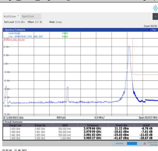
1-N77-3700-3980--30-50-H-5-CP-QPSK-Edge_1RB_Right-1@132-Ant1-PASS-see graph
