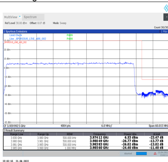
1-N77-3700-3980--30-50-H-3-DFT-PI2BPSK-Outer_Full-128@0-Ant1-PASS-see graph
