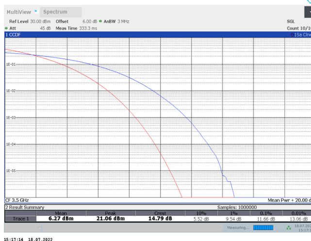
42-42-20MHz-20MHz-QPSK-QPSK-42491-42689-100RB#0-100RB#0
