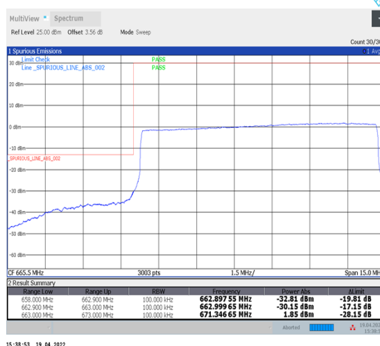
1-N71--15-10-L-6-CP-QPSK-Outer_Full-52@0-Ant1-PASS-see graph
