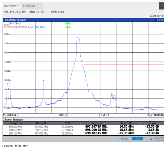
1-N71--15-5-H-2-DFT-PI2BPSK-Edge_1RB_Right-1@24-Ant1-PASS-see graph
