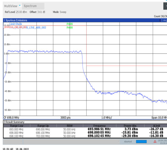
1-N71--15-5-H-3-DFT-PI2BPSK-Outer_Full-25@0-Ant1-PASS-see graph
