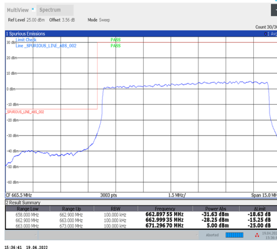
1-N71--15-10-L-3-DFT-PI2BPSK-Outer_Full-50@0-Ant1-PASS-see graph
