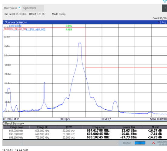
1-N71--15-5-H-5-CP-QPSK-Edge_1RB_Right-1@24-Ant1-PASS-see graph
