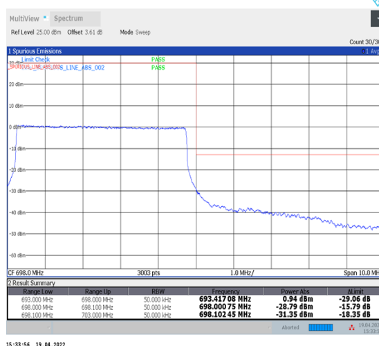
1-N71--15-5-H-6-CP-QPSK-Outer_Full-25@0-Ant1-PASS-see graph
