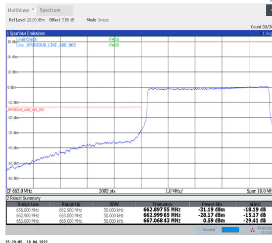
1-N71--15-5-L-6-CP-QPSK-Outer_Full-25@0-Ant1-PASS-see graph
