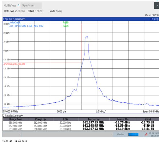
1-N71--15-5-L-1-DFT-PI2BPSK-Edge_1RB_Left-1@0-Ant1-PASS-see graph
