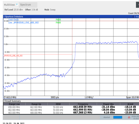
1-N71--15-5-L-3-DFT-PI2BPSK-Outer_Full-25@0-Ant1-PASS-see graph
