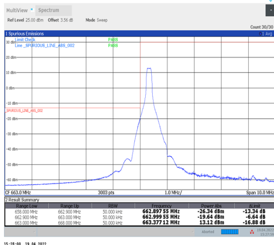
1-N71--15-5-L-4-CP-QPSK-Edge_1RB_Left-1@0-Ant1-PASS-see graph
