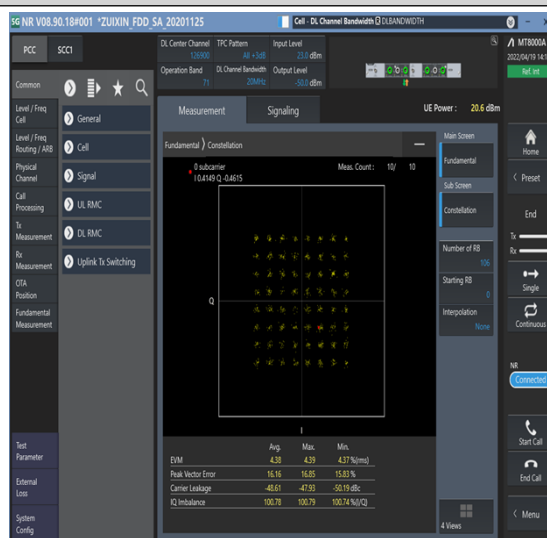
1-N71--15-20-M-8-CP-64QAM-Outer_Full-106@0-Ant1-see graph-PASS
