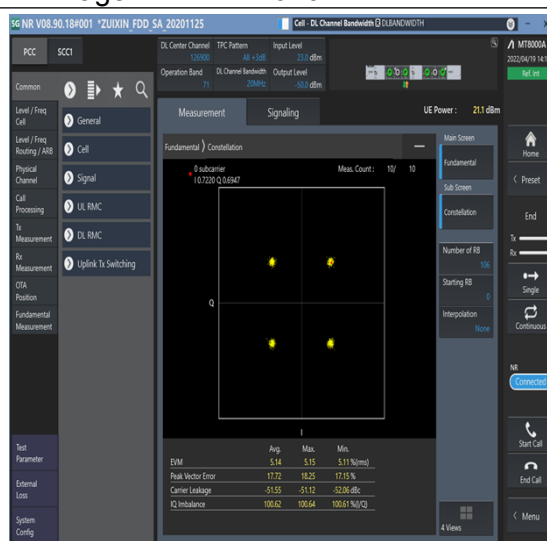
1-N71--15-20-M-6-CP-QPSK-Outer_Full-106@0-Ant1-see graph-PASS
