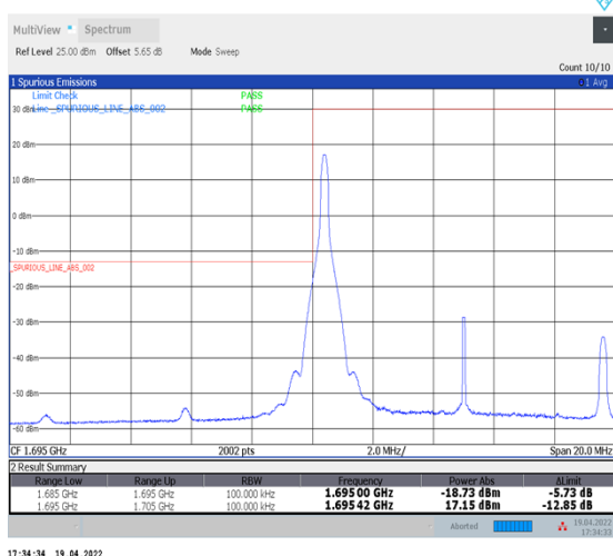
1-N70--15-10-L-4-CP-QPSK-Edge_1RB_Left-1@0-Ant1-seegraph-PASS-see graph
