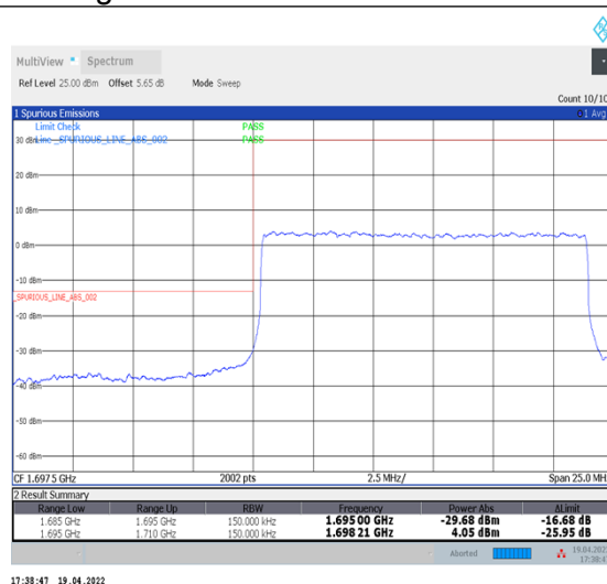
1-N70--15-15-L-3-DFT-PI2BPSK-Outer_Full-75@0-Ant1-seegraph-PASS-see graph
