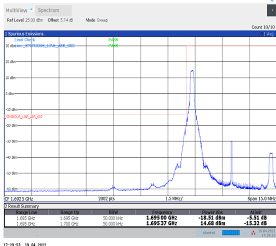
1-N70--15-5-L-4-CP-QPSK-Edge_1RB_Left-1@0-Ant1-seegraph-PASS-see graph
