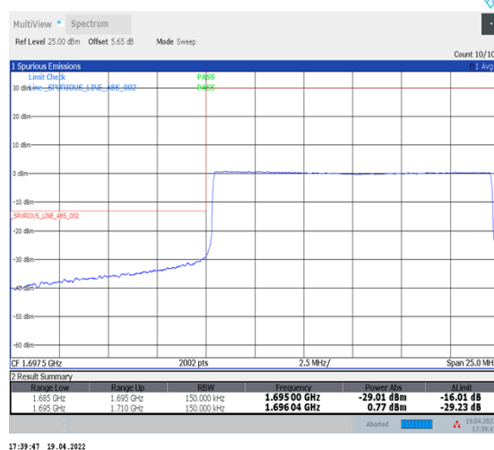
1-N70--15-15-L-6-CP-QPSK-Outer_Full-79@0-Ant1-seegraph-PASS-see graph
