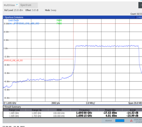
1-N70--15-10-L-3-DFT-PI2BPSK-Outer_Full-50@0-Ant1-seegraph-PASS-see graph
