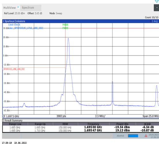
1-N70--15-15-L-4-CP-QPSK-Edge_1RB_Left-1@0-Ant1-seegraph-PASS-see graph
