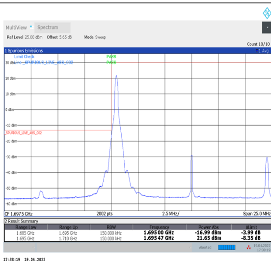
1-N70--15-15-L-1-DFT-PI2BPSK-Edge_1RB_Left-1@0-Ant1-seegraph-PASS-see graph
