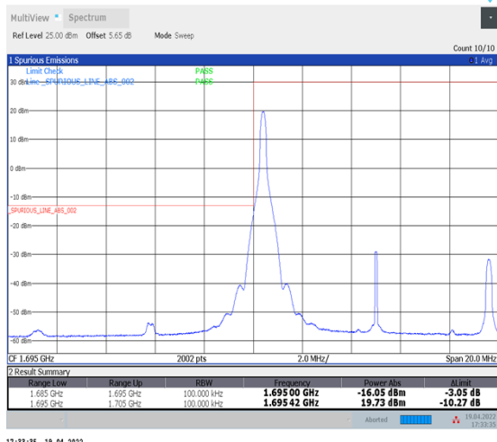
1-N70--15-10-L-1-DFT-PI2BPSK-Edge_1RB_Left-1@0-Ant1-seegraph-PASS-see graph
