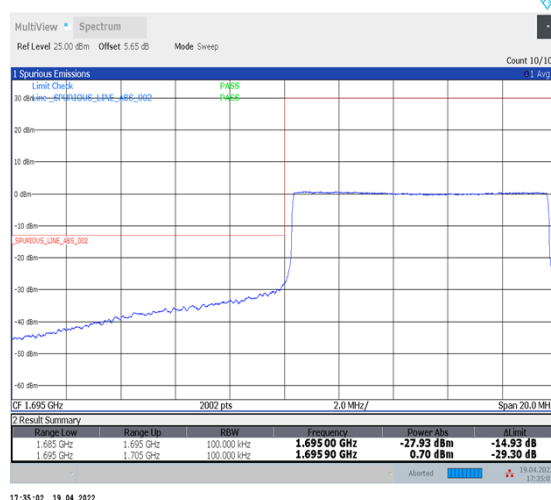
1-N70--15-10-L-6-CP-QPSK-Outer_Full-52@0-Ant1-seegraph-PASS-see graph
