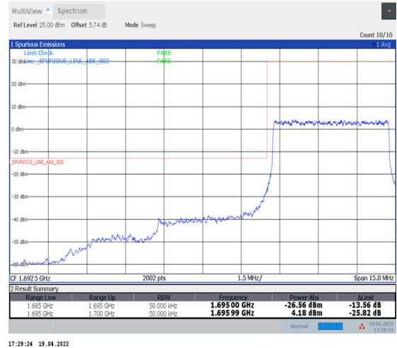
1-N70--15-5-L-3-DFT-PI2BPSK-Outer_Full-25@0-Ant1-seegraph-PASS-see graph
