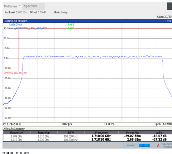
1-N66-PC3-15-10-L-3-DFT-PI2BPSK-Outer_Full-50@0-Ant1-seegraph-PASS-see graph
