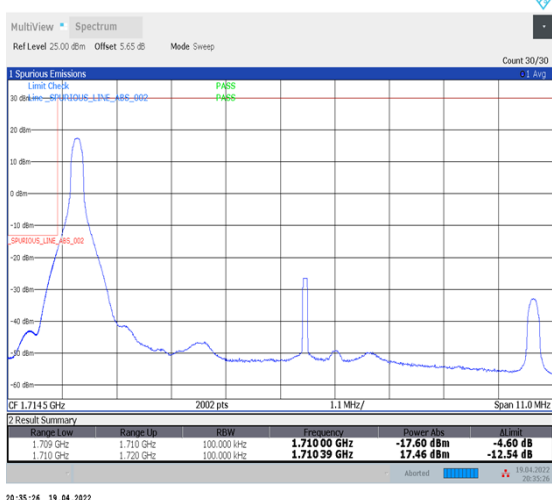
1-N66-PC3-15-10-L-4-CP-QPSK-Edge_1RB_Left-1@0-Ant1-seegraph-PASS-see graph
