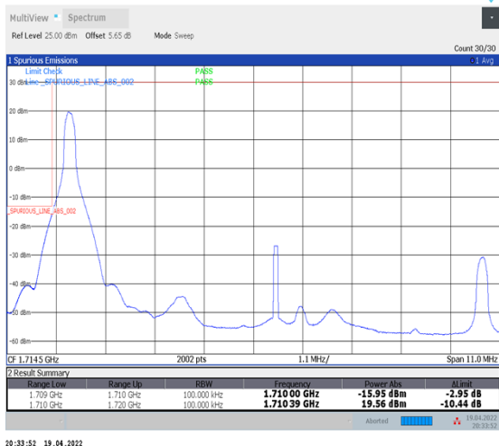
1-N66-PC3-15-10-L-1-DFT-PI2BPSK-Edge_1RB_Left-1@0-Ant1-seegraph-PASS-see graph
