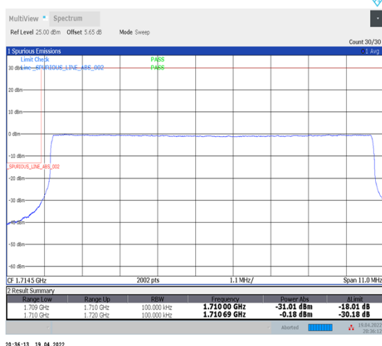
1-N66-PC3-15-10-L-6-CP-QPSK-Outer_Full-52@0-Ant1-seegraph-PASS-see graph
