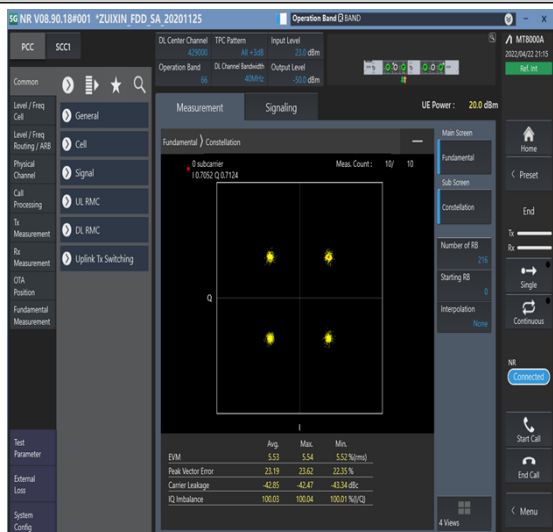
1-N66-PC3-15-40-M-6-CP-QPSK-Outer_Full-216@0-Ant1-see graph-PASS
