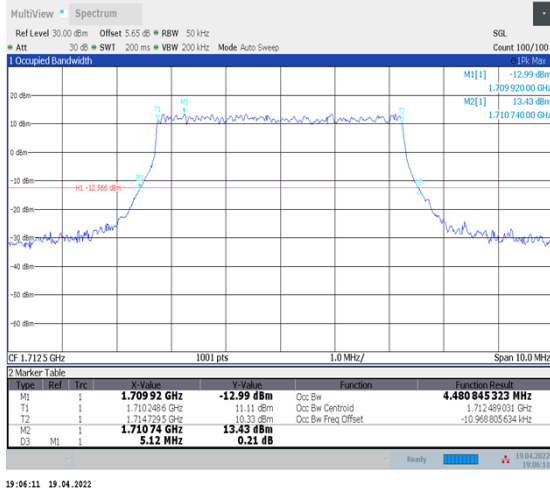
1-N66-PC3-15-5-L-1-DFT-QPSK-Outer_Full-25@0- Ant1-4.481-5.120-≤5-PASS
