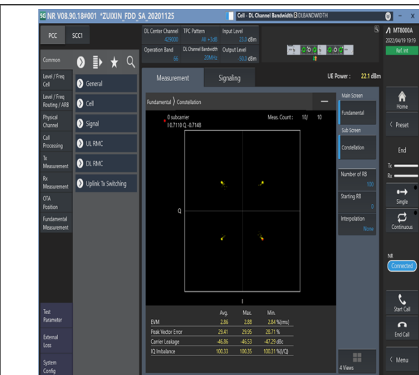
1-N66-PC3-15-20-M-2-DFT-QPSK-Outter_Full-100@0-Ant1-see graph-PASS
