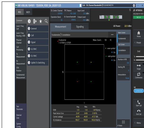
1-N66-PC3-15-20-M-1-DFT-PI2BPSK-Outter_Full-100@0-Ant1-see graph-PASS
