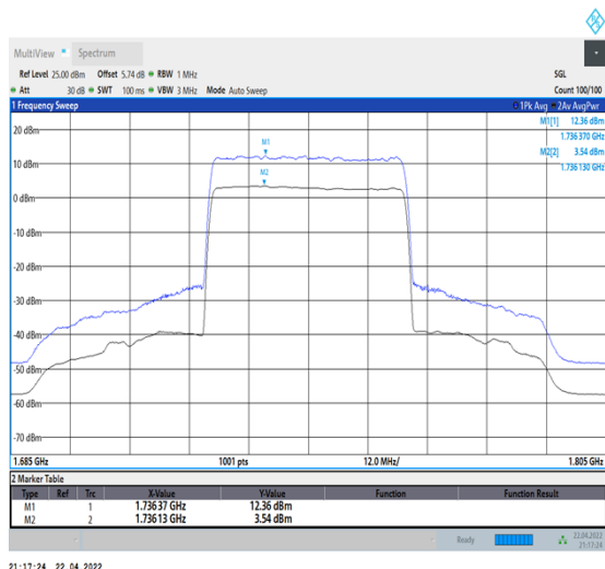
1-N66-PC3-15-40-M-1-DFT-256QAM-Outer_Full-216@0-Ant1-8.82-100%-0.00-8.82-PASS-≤13
