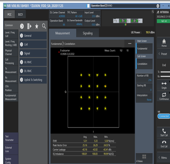
1-N66-PC3-15-40-M-7-CP-16QAM-Outer_Full-216@0-Ant1-see graph-PASS
