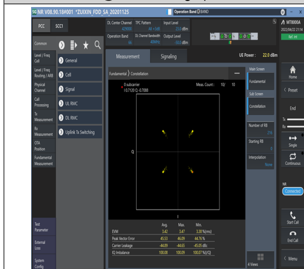
1-N66-PC3-15-40-M-2-DFT-QPSK-Outer_Full-216@0-Ant1-see graph-PASS
