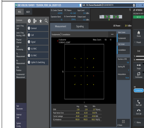
1-N66-PC3-15-20-M-3-DFT-16QAM-Outter_Full-100@0-Ant1-see graph-PASS
