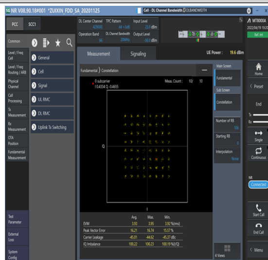
1-N66-PC3-15-20-M-8-CP-64QAM-Outer_Full-106@0-Ant1-see graph-PASS
