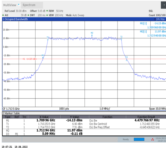
1-N66-PC3-15-5-L-3-DFT-16QAM-Outer_Full-25@0- Ant1-4.48-5.090-≤5-PASS
