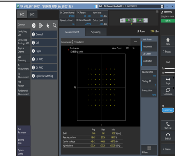
1-N66-PC3-15-20-M-4-DFT-64QAM-Outter_Full-100@0-Ant1-see graph-PASS
