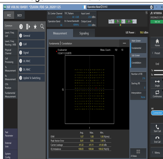
1-N66-PC3-15-40-M-5-DFT-256QAM-Outer_Full-216@0-Ant1-see graph-PASS
