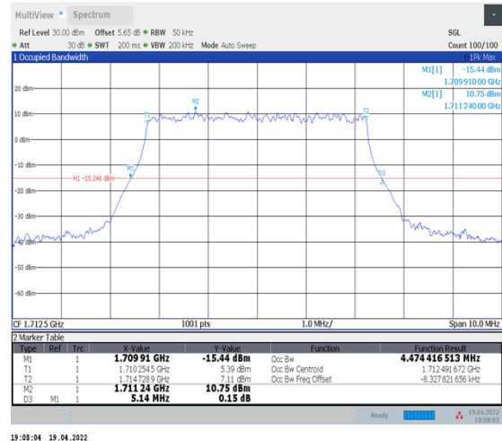
1-N66-PC3-15-5-L-4-DFT-64QAM-Outer_Full-25@0- Ant1-4.474-5.140-≤5-PASS
