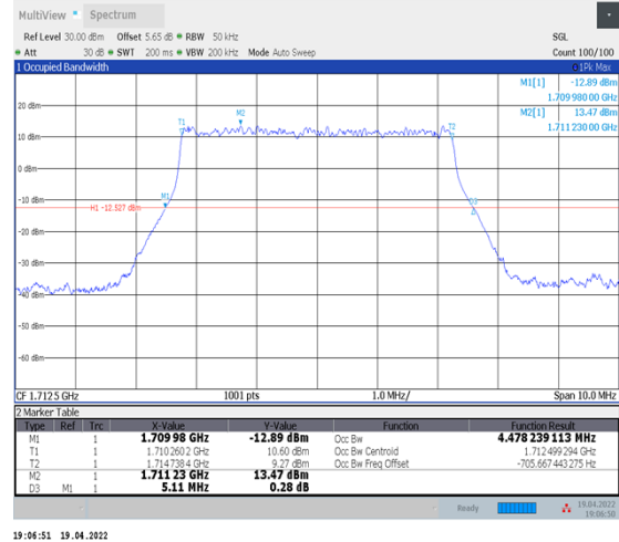
1-N66-PC3-15-5-L-2-DFT-PI2BPSK-Outer_Full- 25@0-Ant1-4.478-5.110-≤5-PASS
