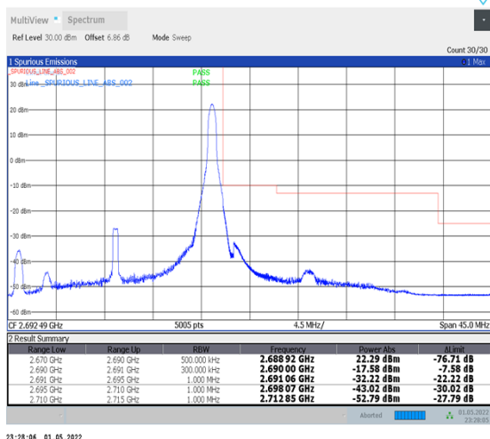
1-N41-PC2-30-20-H-5-CP-QPSK-Edge_1RB_Right-1@50-Ant2-PASS-see graph
