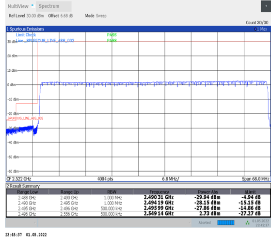
1-N41-PC2-30-60-L-6-CP-QPSK-Outer_Full-162@0-Ant2-PASS-see graph
