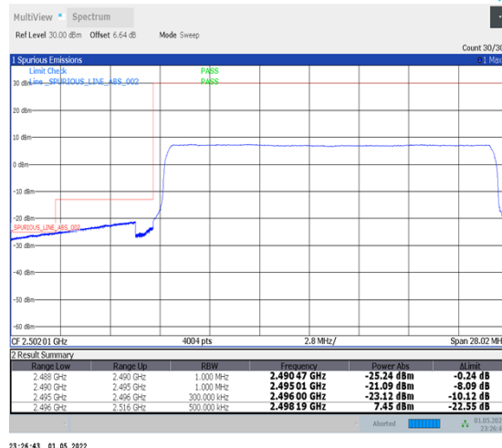
1-N41-PC2-30-20-L-6-CP-QPSK-Outer_Full-51@0-Ant2-PASS-see graph
