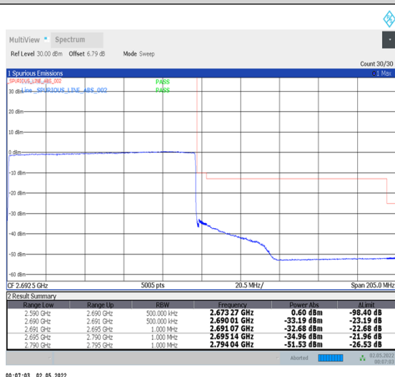
1-N41-PC2-30-100-H-6-CP-QPSK-Outer_Full-273@0-Ant2-PASS-see graph
