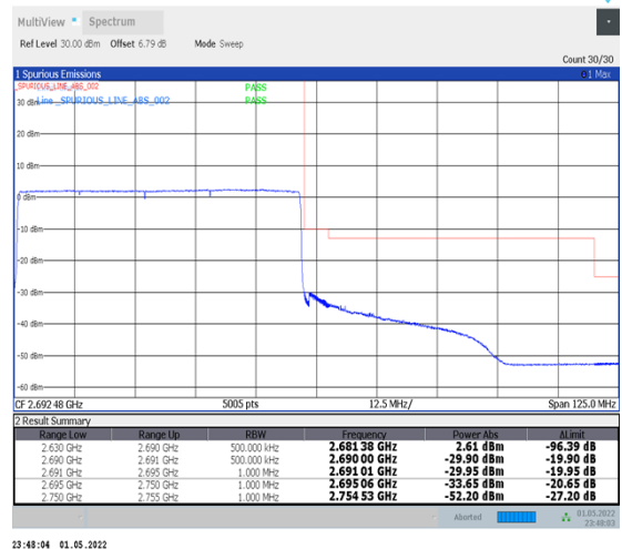
1-N41-PC2-30-60-H-6-CP-QPSK-Outer_Full-162@0-Ant2-PASS-see graph
