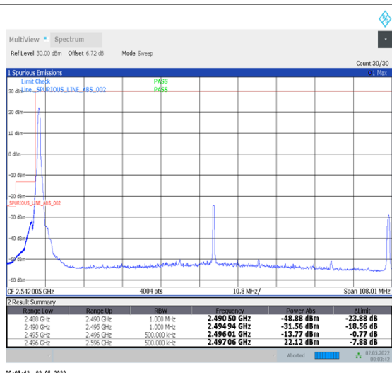
1-N41-PC2-30-100-L-4-CP-QPSK-Edge_1RB_Left-1@0-Ant2-PASS-see graph
