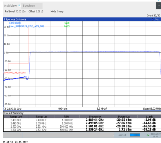
1-N41-PC2-30-70-L-6-CP-QPSK-Outer_Full-189@0-Ant2-PASS-see graph
