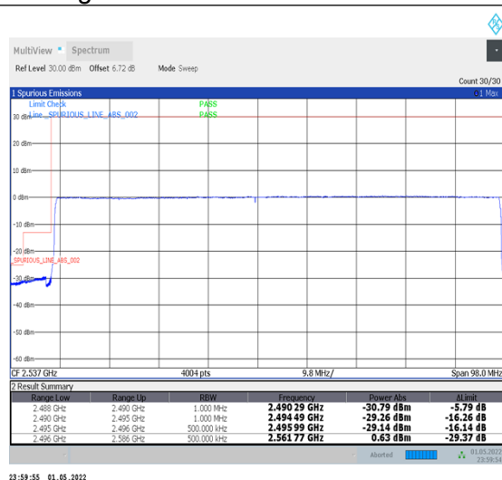
1-N41-PC2-30-90-L-6-CP-QPSK-Outer_Full-245@0-Ant2-PASS-see graph
