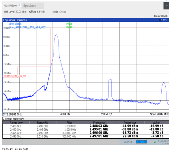
1-N41-PC2-30-20-L-4-CP-QPSK-Edge_1RB_Left-1@0-Ant2-PASS-see graph
