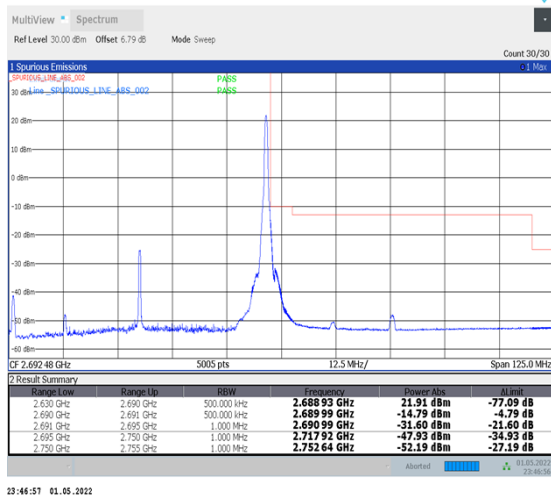
1-N41-PC2-30-60-H-5-CP-QPSK-Edge_1RB_Right-1@161-Ant2-PASS-see graph
