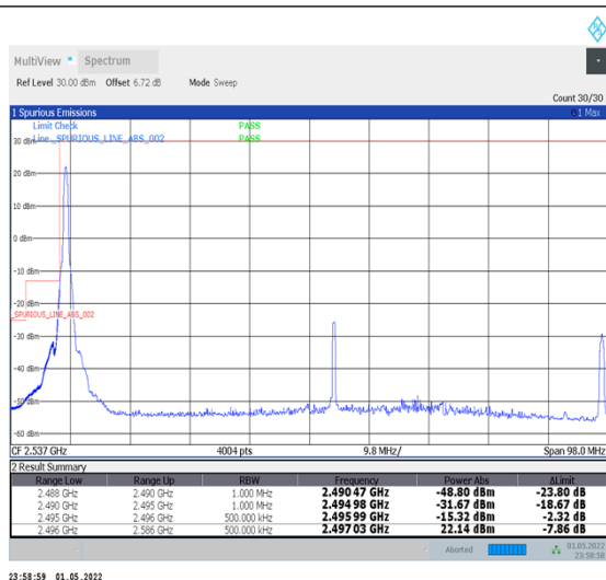
1-N41-PC2-30-90-L-4-CP-QPSK-Edge_1RB_Left-1@0-Ant2-PASS-see graph
