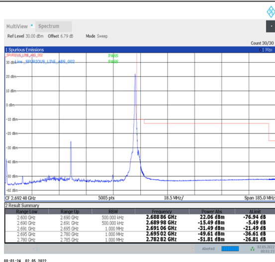
1-N41-PC2-30-90-H-5-CP-QPSK-Edge_1RB_Right-1@244-Ant2-PASS-see graph
