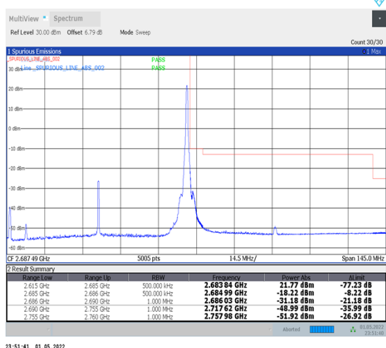
1-N41-PC2-30-70-H-5-CP-QPSK-Edge_1RB_Right-1@188-Ant2-PASS-see graph
