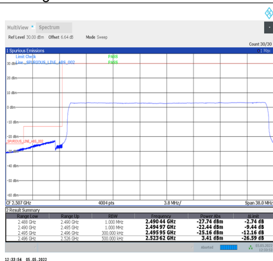
1-N41-PC2-30-30-L-6-CP-QPSK-Outer_Full-78@0-Ant2-PASS-see graph
