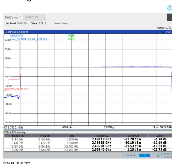
1-N41-PC2-30-80-L-6-CP-QPSK-Outer_Full-217@0-Ant2-PASS-see graph
