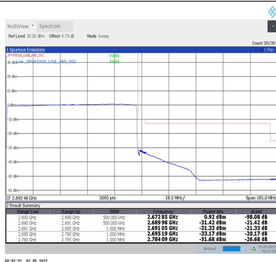
1-N41-PC2-30-90-H-6-CP-QPSK-Outer_Full-245@0-Ant2-PASS-see graph
