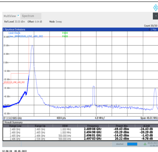
1-N41-PC2-30-40-L-4-CP-QPSK-Edge_1RB_Left-1@0-Ant2-PASS-see graph
