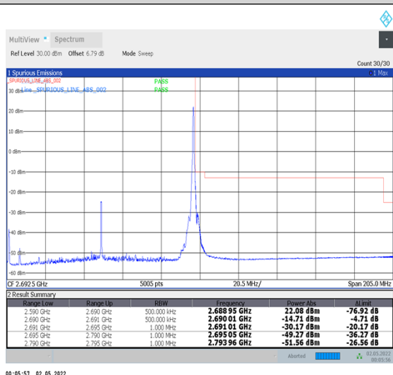
1-N41-PC2-30-100-H-5-CP-QPSK-Edge_1RB_Right-1@272-Ant2-PASS-see graph
