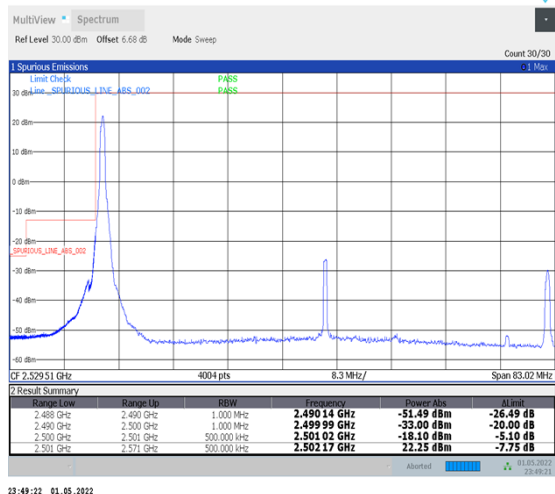
1-N41-PC2-30-70-L-4-CP-QPSK-Edge_1RB_Left-1@0-Ant2-PASS-see graph
