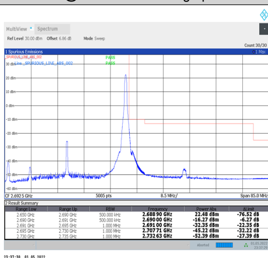
1-N41-PC2-30-40-H-5-CP-QPSK-Edge_1RB_Right-1@105-Ant2-PASS-see graph
