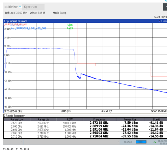
1-N41-PC2-30-20-H-6-CP-QPSK-Outer_Full-51@0-Ant2-PASS-see graph
