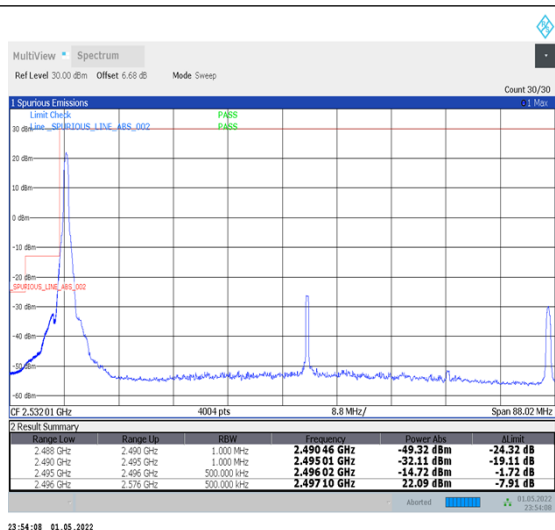
1-N41-PC2-30-80-L-4-CP-QPSK-Edge_1RB_Left-1@0-Ant2-PASS-see graph
