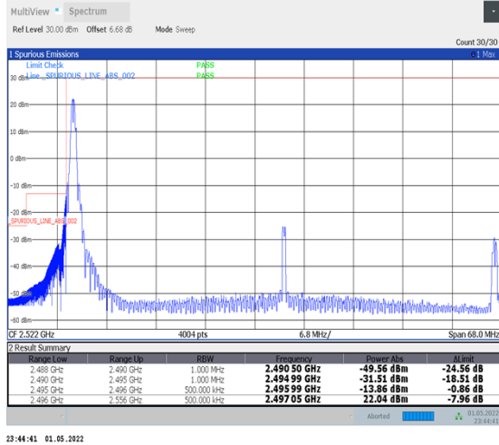
1-N41-PC2-30-60-L-4-CP-QPSK-Edge_1RB_Left-1@0-Ant2-PASS-see graph
