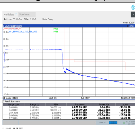
1-N41-PC2-30-30-H-6-CP-QPSK-Outer_Full-78@0-Ant2-PASS-see graph
