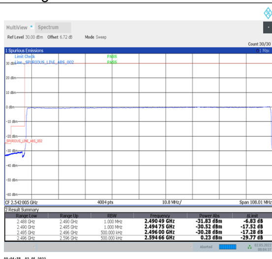
1-N41-PC2-30-100-L-6-CP-QPSK-Outer_Full-273@0-Ant2-PASS-see graph
