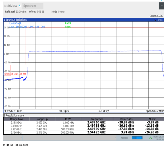
1-N41-PC2-30-50-L-6-CP-QPSK-Outer_Full-133@0-Ant2-PASS-see graph
