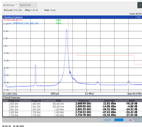
1-N41--30-40-H-2-DFT-PI2BPSK-Edge_1RB_Right-1@105-Ant1-PASS-see graph
