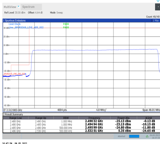
1-N41--30-40-L-6-CP-QPSK-Outer_Full-106@0-Ant1-PASS-see graph
