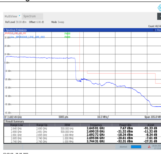
1-N41--30-50-H-3-DFT-PI2BPSK-Outer_Full-128@0-Ant1-PASS-see graph
