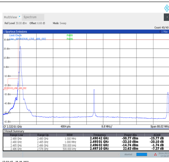
1-N41--30-80-L-1-DFT-PI2BPSK-Edge_1RB_Left-1@0-Ant1-PASS-see graph
