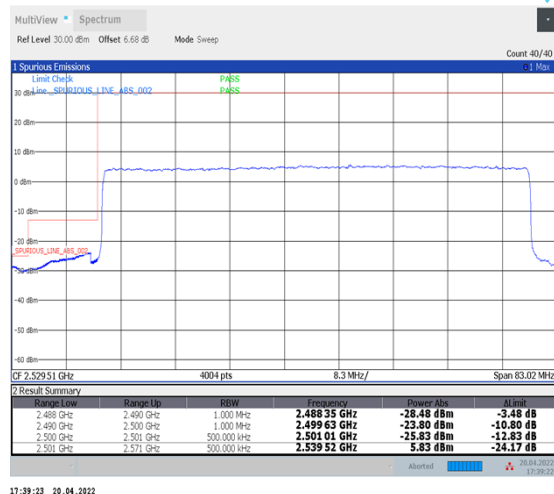
1-N41--30-70-L-3-DFT-PI2BPSK-Outer_Full-180@0-Ant1-PASS-see graph
