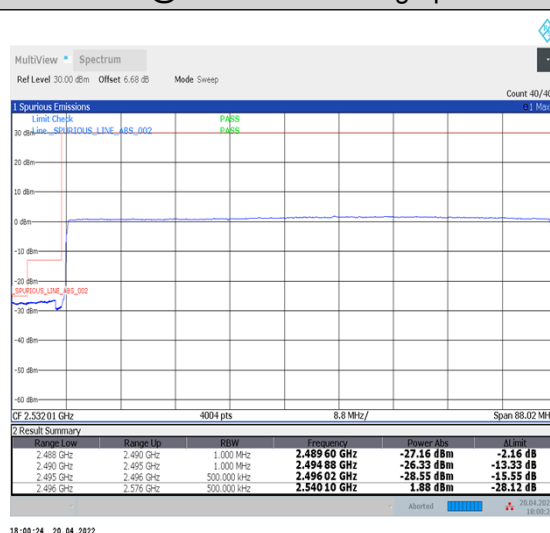
1-N41--30-80-L-6-CP-QPSK-Outer_Full-217@0-Ant1-PASS-see graph
