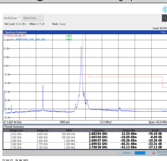
1-N41--30-70-H-5-CP-QPSK-Edge_1RB_Right-1@188-Ant1-PASS-see graph
