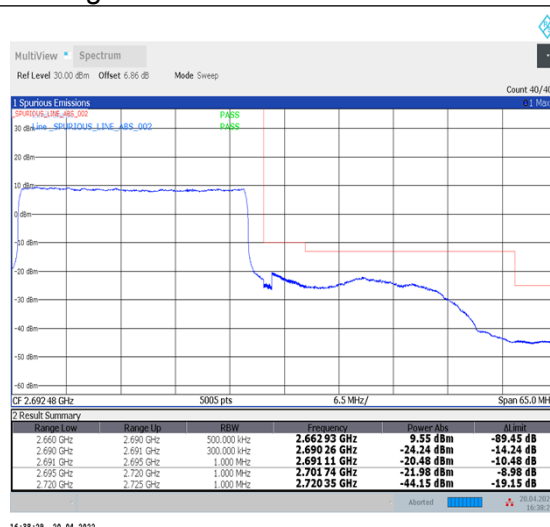
1-N41--30-30-H-3-DFT-PI2BPSK-Outer_Full-75@0-Ant1-PASS-see graph
