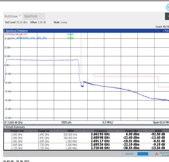
1-N41--30-30-H-6-CP-QPSK-Outer_Full-78@0-Ant1-PASS-see graph
