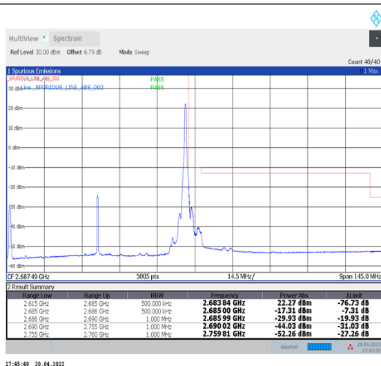
1-N41--30-70-H-2-DFT-PI2BPSK-Edge_1RB_Right-1@188-Ant1-PASS-see graph
