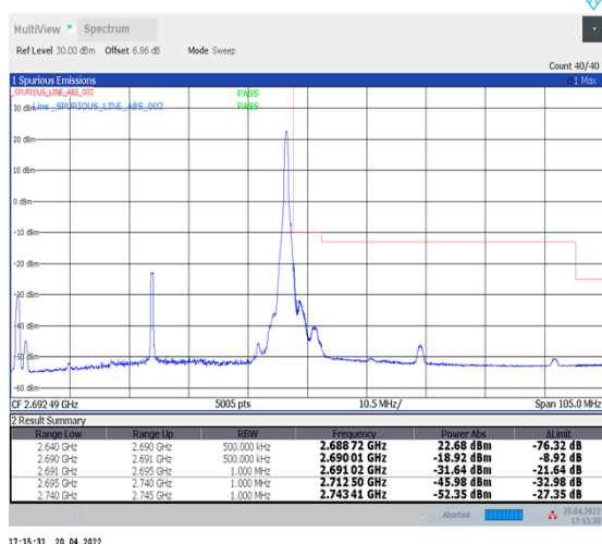
1-N41--30-50-H-5-CP-QPSK-Edge_1RB_Right-1@132-Ant1-PASS-see graph
