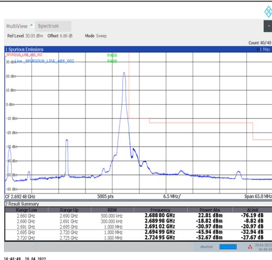
1-N41--30-30-H-5-CP-QPSK-Edge_1RB_Right-1@77-Ant1-PASS-see graph
