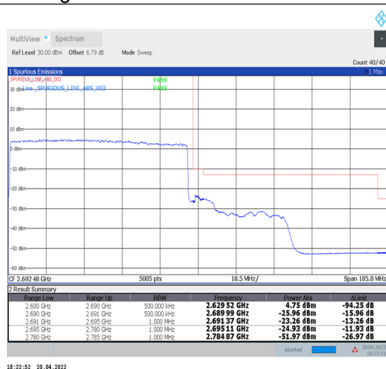
1-N41--30-90-H-3-DFT-PI2BPSK-Outer_Full-240@0-Ant1-PASS-see graph
