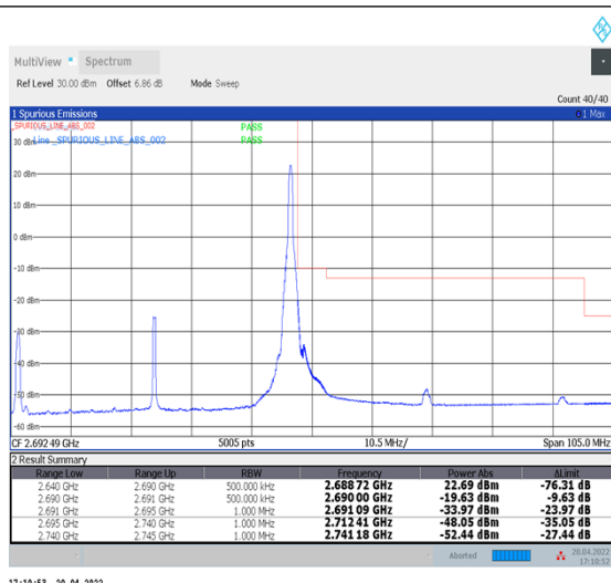
1-N41--30-50-H-2-DFT-PI2BPSK-Edge_1RB_Right-1@132-Ant1-PASS-see graph
