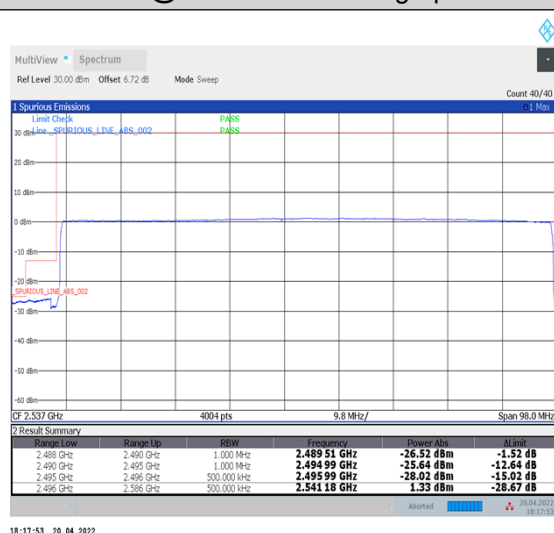
1-N41--30-90-L-6-CP-QPSK-Outer_Full-245@0-Ant1-PASS-see graph
