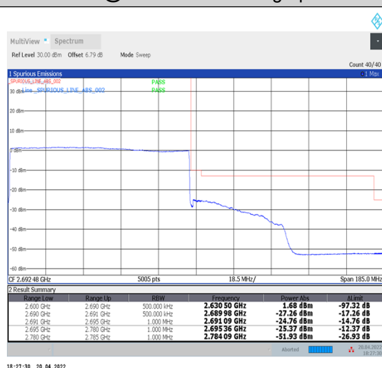
1-N41--30-90-H-6-CP-QPSK-Outer_Full-245@0-Ant1-PASS-see graph
