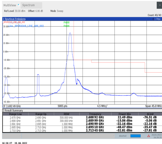
1-N41--30-20-H-2-DFT-PI2BPSK-Edge_1RB_Right-1@50-Ant1-PASS-see graph
