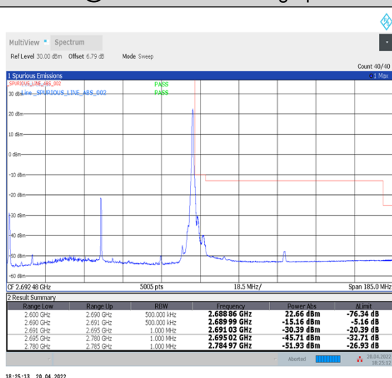
1-N41--30-90-H-5-CP-QPSK-Edge_1RB_Right-1@244-Ant1-PASS-see graph
