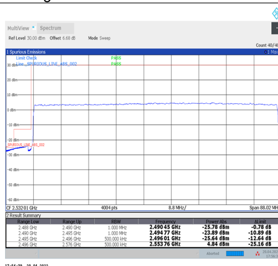
1-N41--30-80-L-3-DFT-PI2BPSK-Outer_Full-216@0-Ant1-PASS-see graph
