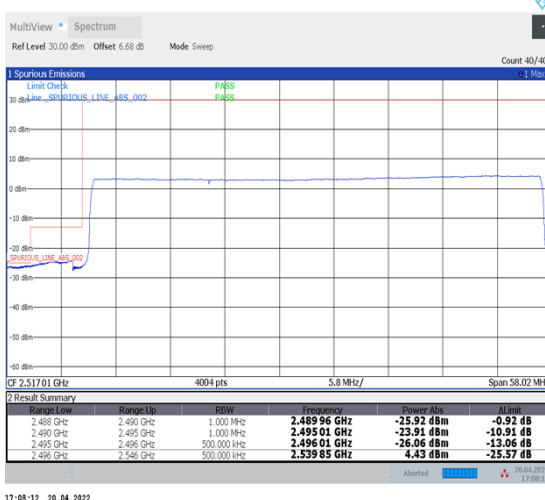
1-N41--30-50-L-6-CP-QPSK-Outer_Full-133@0-Ant1-PASS-see graph
