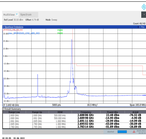
1-N41--30-90-H-2-DFT-PI2BPSK-Edge_1RB_Right-1@244-Ant1-PASS-see graph
