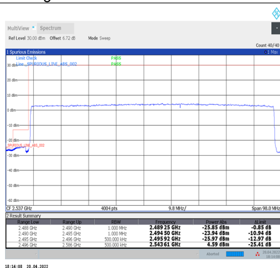
1-N41--30-90-L-3-DFT-PI2BPSK-Outer_Full-240@0-Ant1-PASS-see graph
