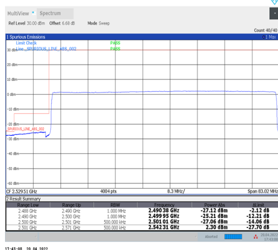
1-N41--30-70-L-6-CP-QPSK-Outer_Full-189@0-Ant1-PASS-see graph
