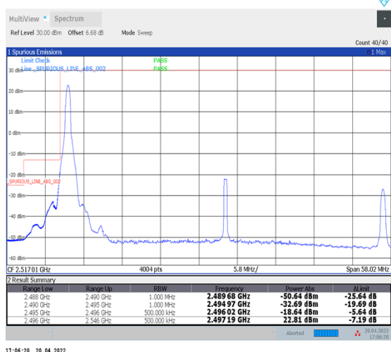
1-N41--30-50-L-4-CP-QPSK-Edge_1RB_Left-1@0-Ant1-PASS-see graph
