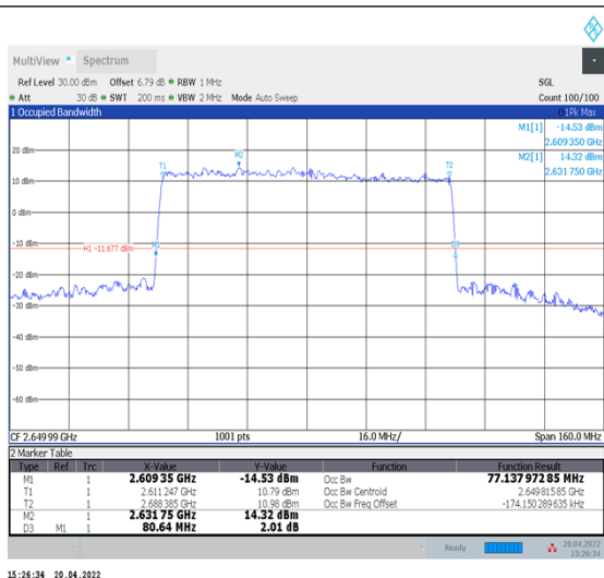
1-N41--30-80-H-5-DFT-256QAM-Outer_Full-216@0-Ant1-77.138-80.640-≤80-PASS
