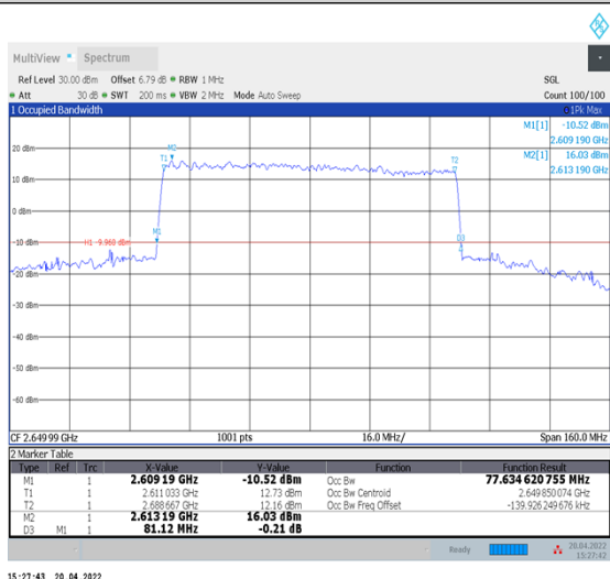
1-N41--30-80-H-7-CP-16QAM-Outer_Full-217@0-Ant1-77.635-81.120-≤80-PASS
