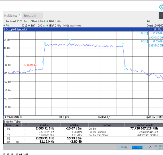
1-N41--30-80-H-8-CP-64QAM-Outer_Full-217@0-Ant1-77.42-81.120-≤80-PASS
