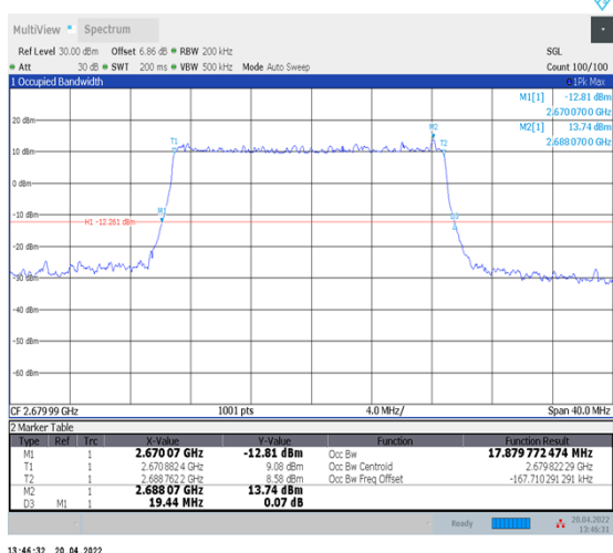
1-N41--30-20-H-5-DFT-256QAM-Outer_Full-50@0-Ant1-17.88-19.440-≤20-PASS
