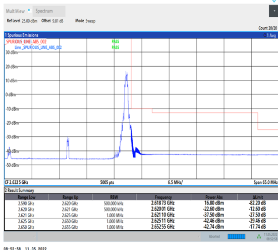
1-N38-PC2-30-30-H-5-CP-QPSK-Edge_1RB_Right-1@77-Ant1-PASS-see graph
