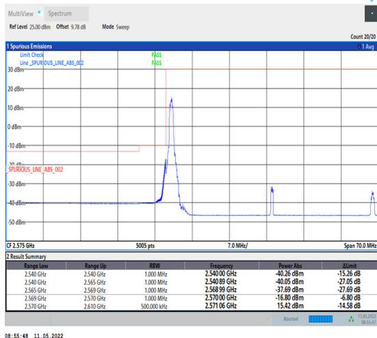
1-N38-PC2-30-40-L-4-CP-QPSK-Edge_1RB_Left-1@0-Ant1-PASS-see graph
