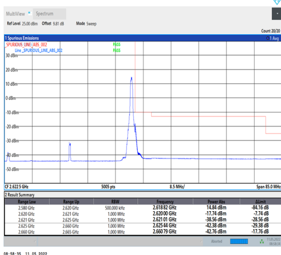
1-N38-PC2-30-40-H-5-CP-QPSK-Edge_1RB_Right-1@105-Ant1-PASS-see graph
