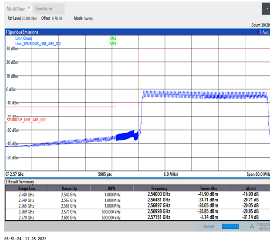
1-N38-PC2-30-30-L-6-CP-QPSK-Outer_Full-78@0-Ant1-PASS-see graph
