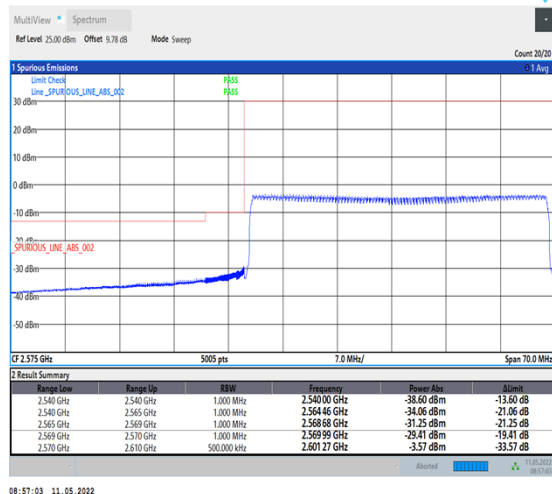
1-N38-PC2-30-40-L-6-CP-QPSK-Outer_Full-106@0-Ant1-PASS-see graph
