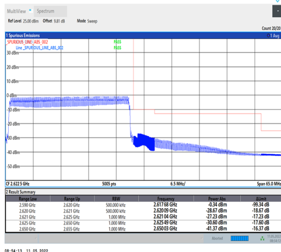
1-N38-PC2-30-30-H-6-CP-QPSK-Outer_Full-78@0-Ant1-PASS-see graph
