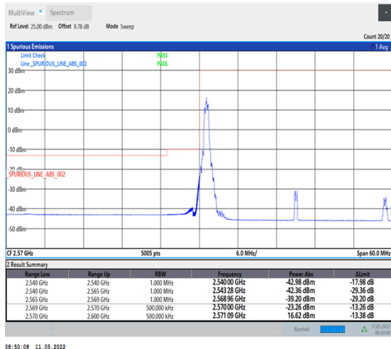
1-N38-PC2-30-30-L-4-CP-QPSK-Edge_1RB_Left-1@0-Ant1-PASS-see graph
