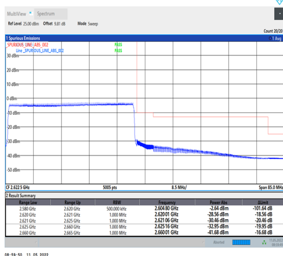
1-N38-PC2-30-40-H-6-CP-QPSK-Outer_Full-106@0-Ant1-PASS-see graph
