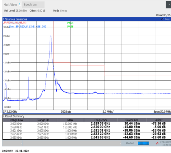
1-N38--30-15-H-2-DFT-PI2BPSK-Edge_1RB_Right-1@37-Ant1-PASS-see graph
