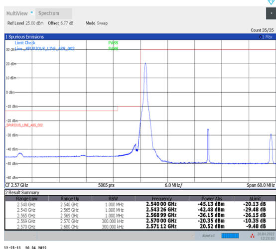
1-N38--30-30-L-4-CP-QPSK-Edge_1RB_Left-1@0-Ant1-PASS-see graph
