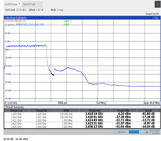
1-N38--30-15-H-3-DFT-PI2BPSK-Outer_Full-36@0-Ant1-PASS-see graph
