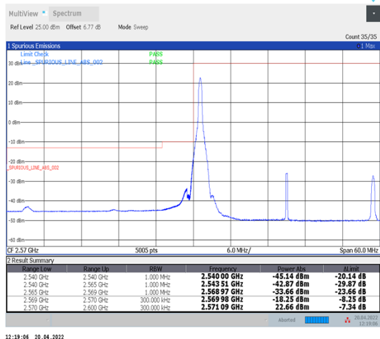
1-N38--30-30-L-1-DFT-PI2BPSK-Edge_1RB_Left-1@0-Ant1-PASS-see graph
