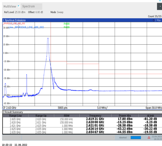
1-N38--30-15-H-5-CP-QPSK-Edge_1RB_Right-1@37-Ant1-PASS-see graph
