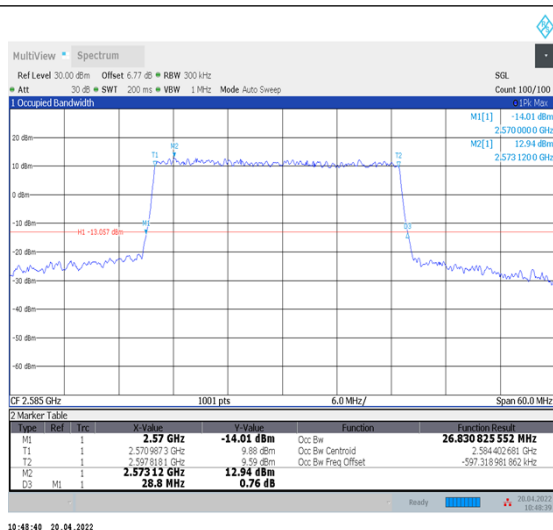
1-N38--30-30-L-4-DFT-64QAM-Outer_Full-75@0- Ant1-26.831-28.800-≤30-PASS
