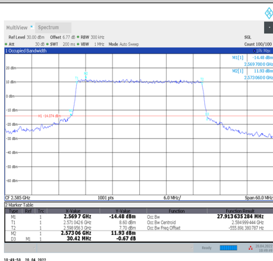
1-N38--30-30-L-6-CP-QPSK-Outer_Full-78@0-Ant1- 27.914-30.420-≤30-PASS
