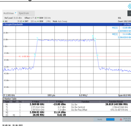
1-N38--30-30-L-5-DFT-256QAM-Outer_Full-75@0- Ant1-26.819-28.980-≤30-PASS
