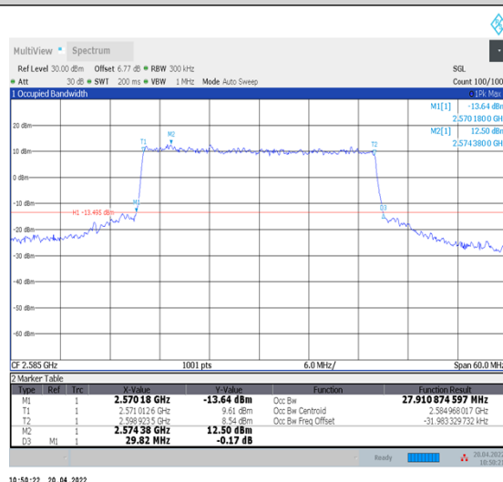
1-N38--30-30-L-7-CP-16QAM-Outer_Full-78@0- Ant1-27.911-29.820-≤30-PASS
