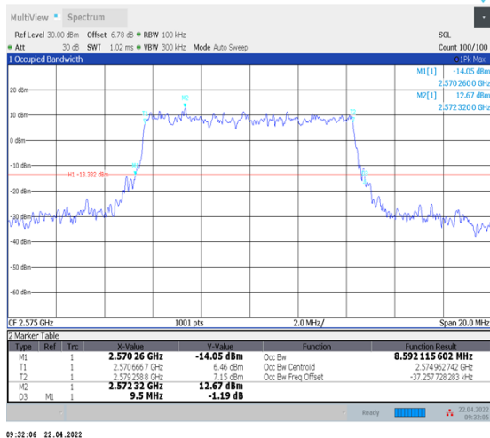
1-N38--30-10-L-3-DFT-16QAM-Outet_Full-24@0- Ant1-8.592-9.500-≤10-PASS
