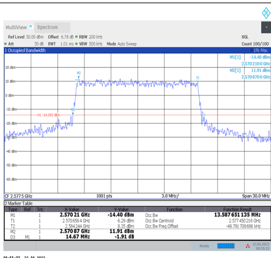
1-N38--30-15-L-6-CP-QPSK-Outet_Full-38@0-Ant1-13.588-14.670-≤15-PASS
