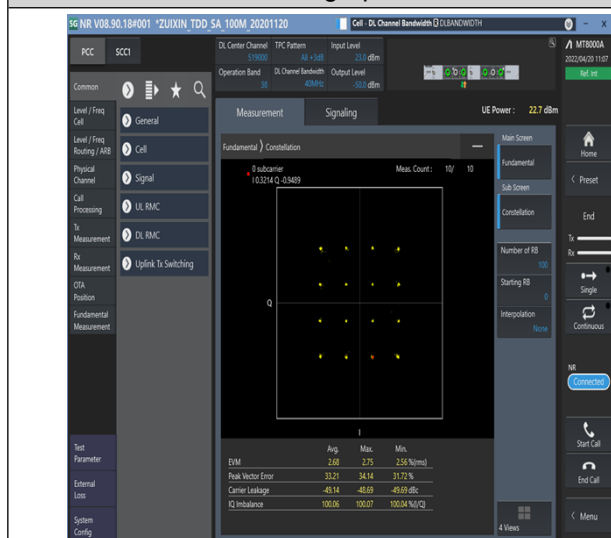
1-N38--30-40-M-3-DFT-16QAM-Outter_Full-100@0- Ant1-see graph-PASS
