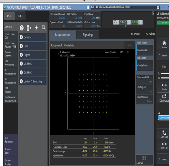
1-N38--30-40-M-4-DFT-64QAM-Outter_Full-100@0- Ant1-see graph-PASS
