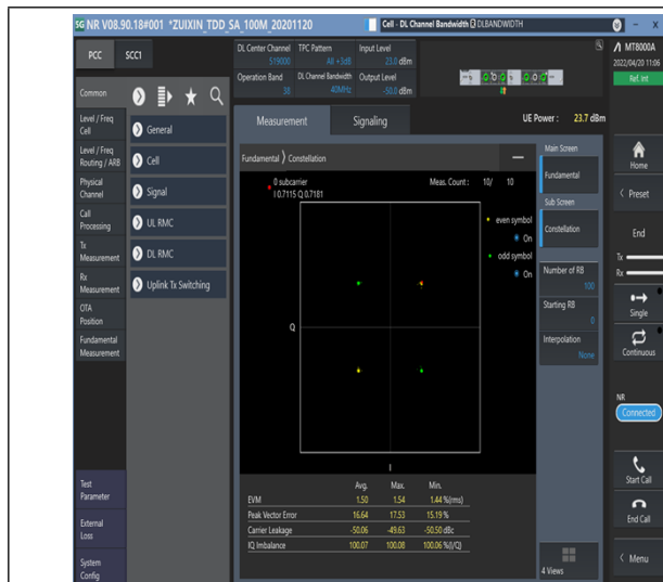
1-N38--30-40-M-1-DFT-PI2BPSK-Outter_Full-100@0- Ant1-see graph-PASS
