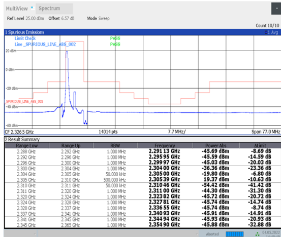
1-N30--15-5-L-4-CP-QPSK-Edge_1RB_Left-1@0-Ant1-PASS-see graph
