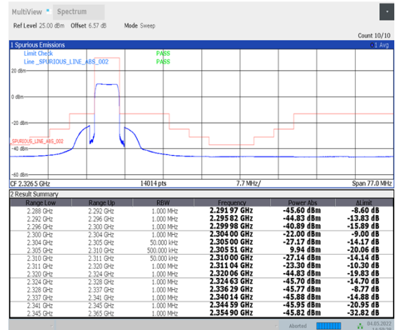
1-N30--15-5-L-6-CP-QPSK-Outer_Full-25@0-Ant1-PASS-see graph
