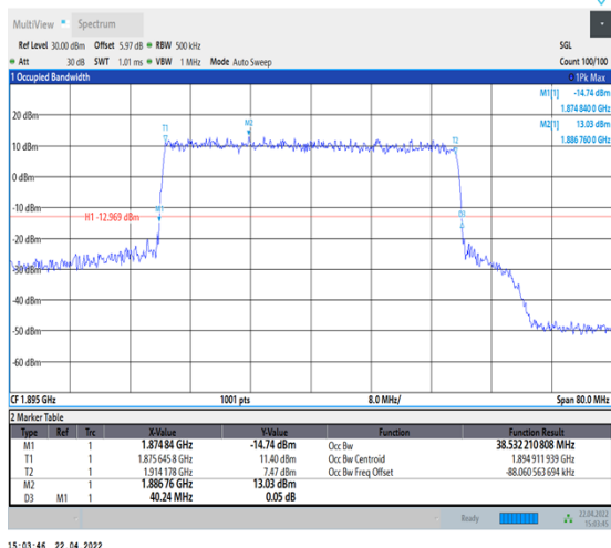
1-N25--15-40-H-3-DFT-16QAM-Outer_Full-216@0-Ant1-38.532-40.240-≤40-PASS
