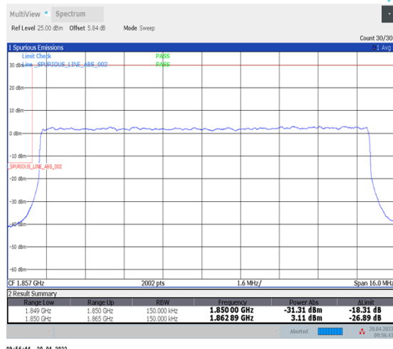
1-N25--15-15-L-3-DFT-PI2BPSK-Outer_Full-75@0-Ant1-seegraph-PASS-see graph
