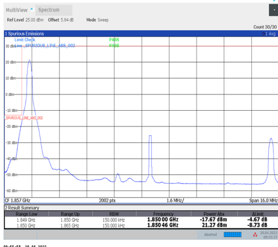
1-N25--15-15-L-1-DFT-PI2BPSK-Edge_1RB_Left-1@0-Ant1-seegraph-PASS-see graph
