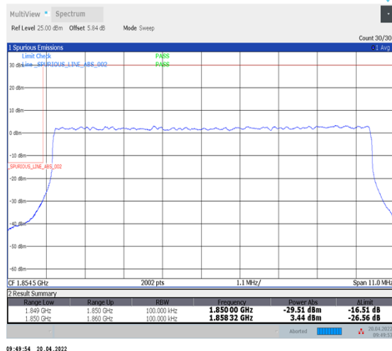
1-N25--15-10-L-3-DFT-PI2BPSK-Outer_Full-50@0-Ant1-seegraph-PASS-see graph
