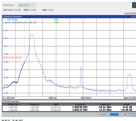
1-N25--15-5-L-4-CP-QPSK-Edge_1RB_Left-1@0-Ant1-seegraph-PASS-see graph
