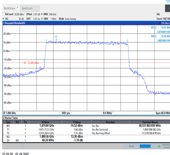
1-N25--15-40-H-7-CP-16QAM-Outer_Full-216@0-Ant1-38.552-40.240-≤40-PASS
