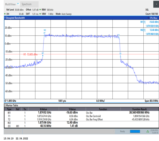
1-N25--15-40-H-6-CP-QPSK-Outer_Full-216@0-Ant1-38.56-40.160-≤40-PASS
