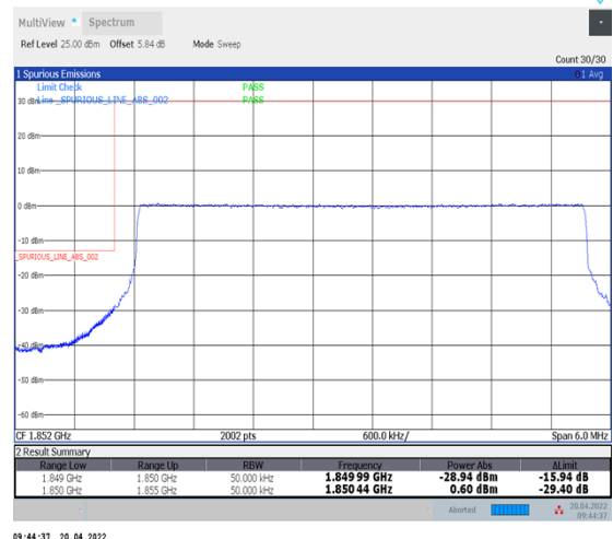
1-N25--15-5-L-6-CP-QPSK-Outer_Full-25@0-Ant1-seegraph-PASS-see graph
