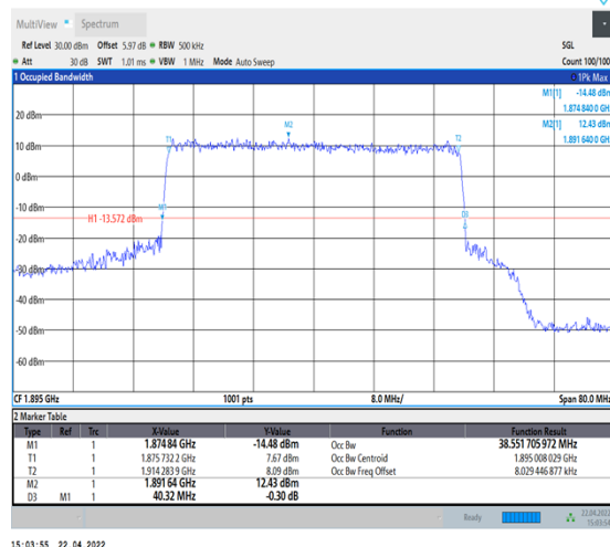
1-N25--15-40-H-4-DFT-64QAM-Outer_Full-216@0-Ant1-38.552-40.320-≤40-PASS
