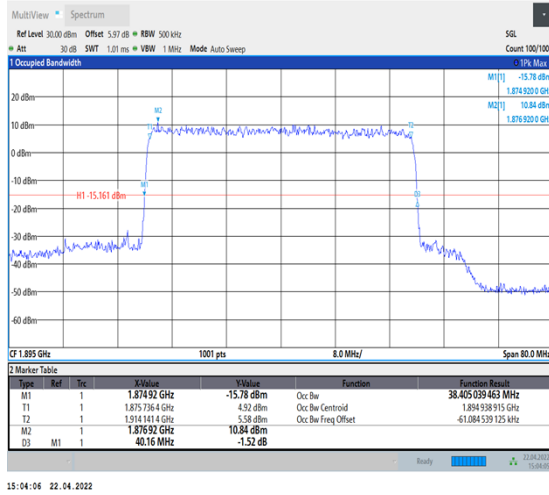
1-N25--15-40-H-5-DFT-256QAM-Outer_Full-216@0-Ant1-38.405-40.160-≤40-PASS
