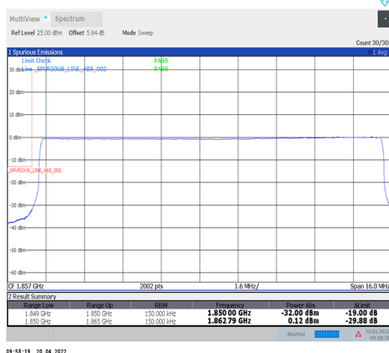
1-N25--15-15-L-6-CP-QPSK-Outer_Full-79@0-Ant1-seegraph-PASS-see graph
