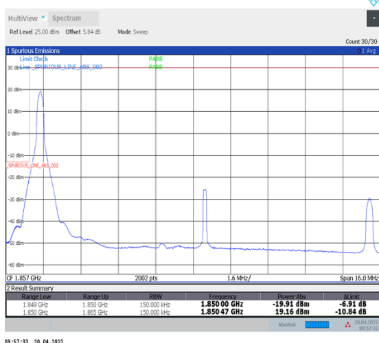
1-N25--15-15-L-4-CP-QPSK-Edge_1RB_Left-1@0-Ant1-seegraph-PASS-see graph
