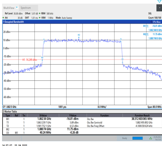
1-N25--15-40-M-8-CP-64QAM-Outer_Full-216@0-Ant1-38.512-40.240-≤40-PASS
