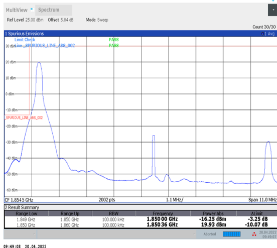
1-N25--15-10-L-1-DFT-PI2BPSK-Edge_1RB_Left-1@0-Ant1-seegraph-PASS-see graph
