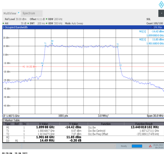
1-N25--15-15-H-3-DFT-16QAM-Outer_Full-75@0- Ant1-13.441-14.490-≤15-PASS
