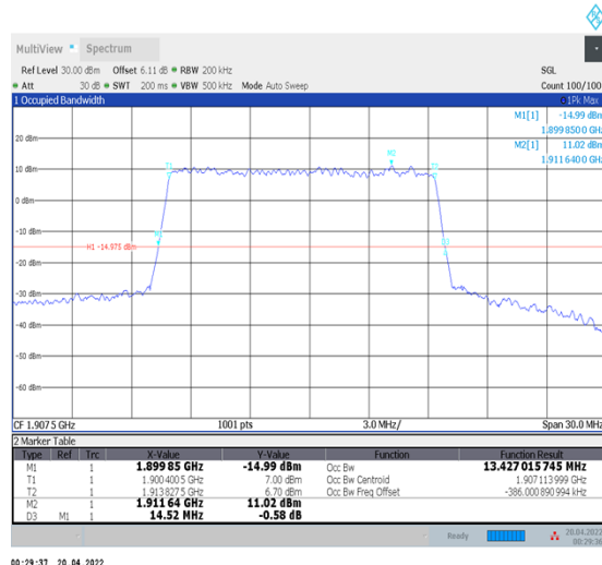
1-N25--15-15-H-4-DFT-64QAM-Outer_Full-75@0- Ant1-13.427-14.520-≤15-PASS
