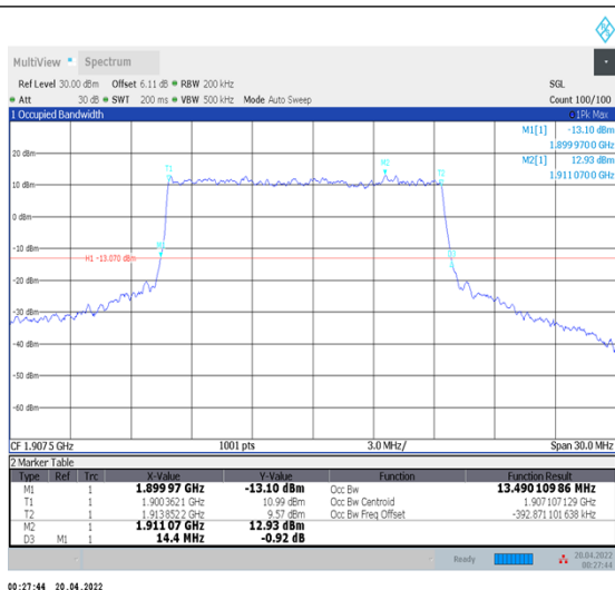
1-N25--15-15-H-1-DFT-QPSK-Outer_Full-75@0- Ant1-13.49-14.400-≤15-PASS
