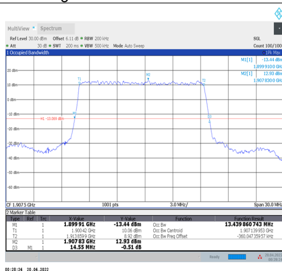
1-N25--15-15-H-2-DFT-PI2BPSK-Outer_Full-75@0- Ant1-13.44-14.550-≤15-PASS
