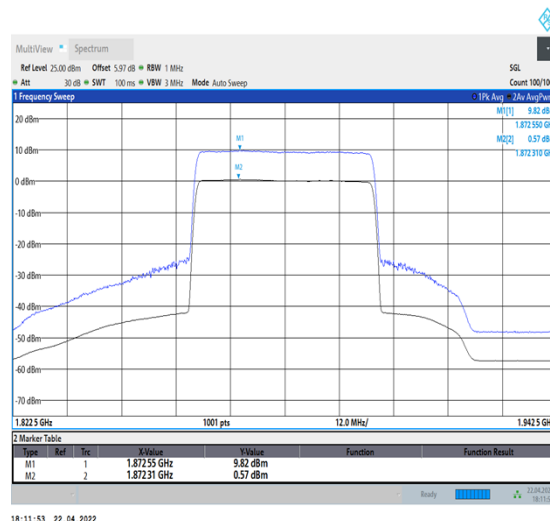
1-N25--15-40-M-2-CP-256QAM-Outer_Full-216@0- Ant1-9.25-100%-0.00-9.25-PASS-≤13
