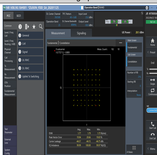
1-N25--15-40-M-4-DFT-64QAM-Outer_Full-216@0- Ant1-see graph-PASS
