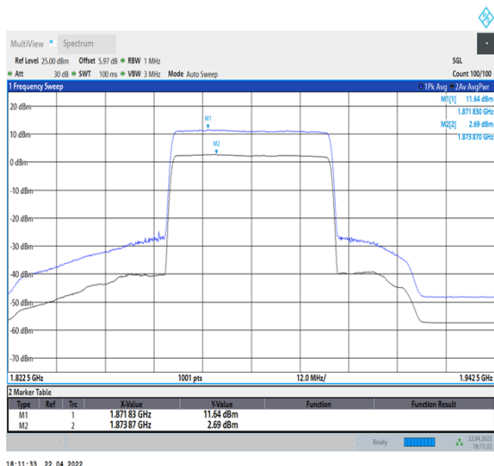
1-N25--15-40-M-1-DFT-256QAM-Outer_Full-216@0- Ant1-8.95-100%-0.00-8.95-PASS-≤13
