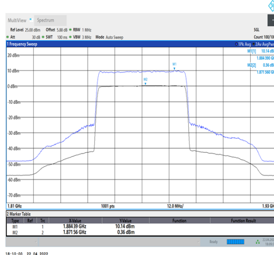
1-N25--15-40-L-2-CP-256QAM-Outer_Full-216@0- Ant1-9.78-100%-0.00-9.78-PASS-≤13
