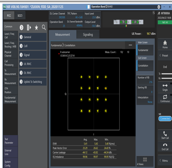
1-N25--15-40-M-7-CP-16QAM-Outer_Full-216@0-Ant1-see graph-PASS
