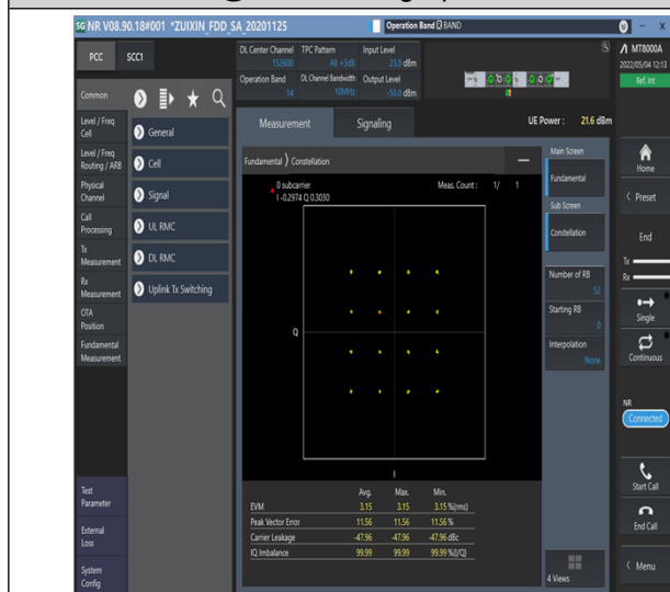
1-N14-PC3-15-10-M-7-CP-16QAM-Outer_Full-52@0-Ant1-see graph-PASS
