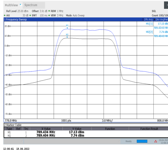
1-N14--15-10-M-2-CP-256QAM-Outer_Full-52@0- Ant1-9.39-100%-0.00-9.39-PASS-≤13
