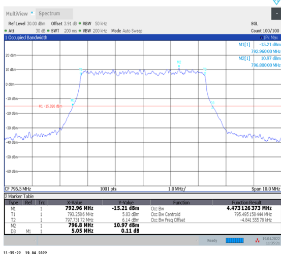
1-N14--15-5-H-5-DFT-256QAM-Outer_Full-25@0-Ant1-4.473-5.050-≤5-PASS
