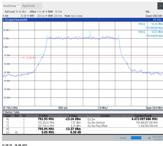
1-N14--15-5-H-3-DFT-16QAM-Outer_Full-25@0-Ant1-4.472-5.050-≤5-PASS
