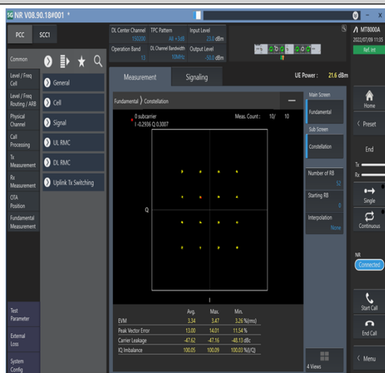
1-N13--15-10-M-7-CP-16QAM-Outer_Full-52@0-Ant1-see graph-PASS
