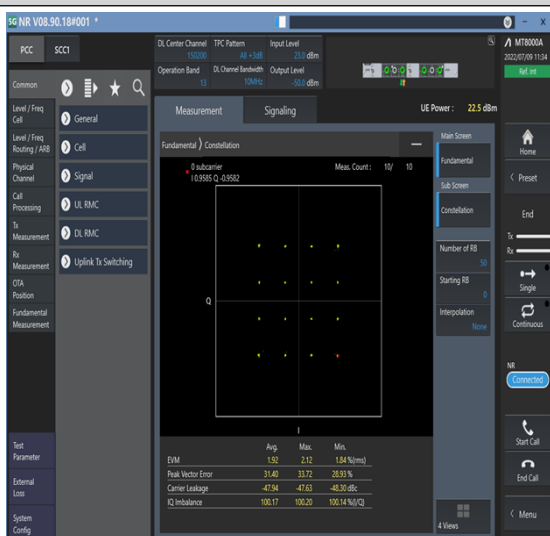
1-N13--15-10-M-3-DFT-16QAM-Outter_Full-50@0- Ant1-see graph-PASS
