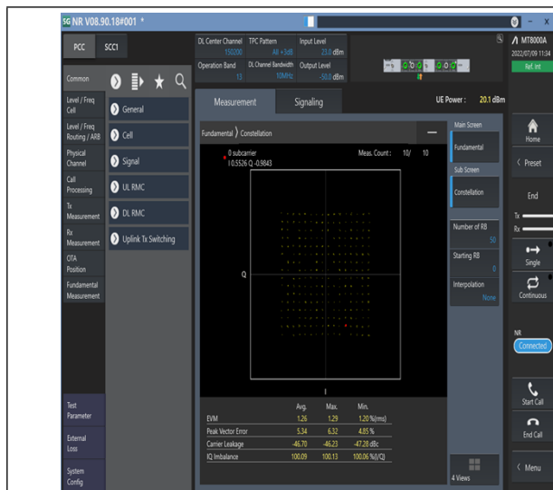
1-N13--15-10-M-5-DFT-256QAM-Outer_Full-50@0-Ant1-see graph-PASS
