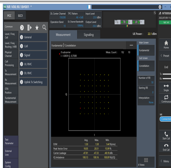
1-N13--15-10-M-4-DFT-64QAM-Outter_Full-50@0- Ant1-see graph-PASS
