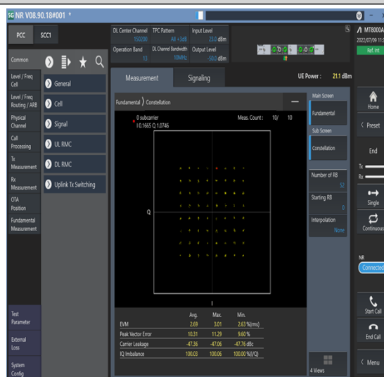
1-N13--15-10-M-8-CP-64QAM-Outer_Full-52@0-Ant1-see graph-PASS
