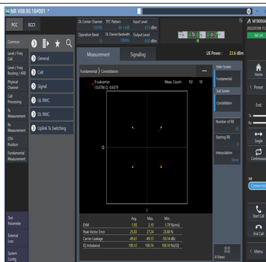
1-N13--15-10-M-2-DFT-QPSK-Outter_Full-50@0- Ant1-see graph-PASS
