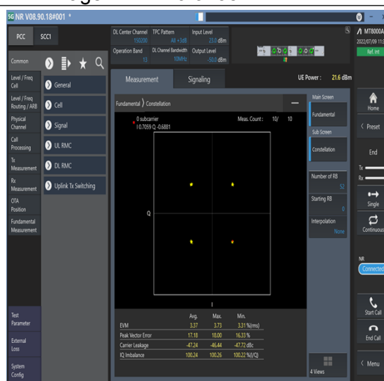
1-N13--15-10-M-6-CP-QPSK-Outer_Full-52@0-Ant1-see graph-PASS
