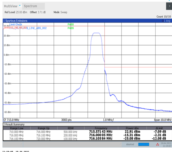
1-N12--15-15-H-2-DFT-PI2BPSK-Edge_1RB_Right-1@78-Ant1-PASS-see graph
