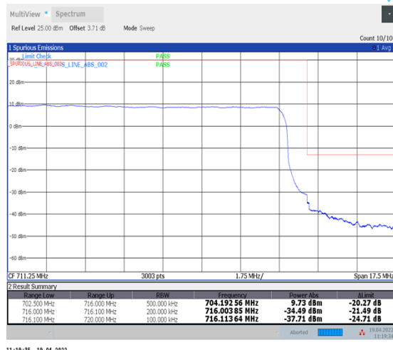
1-N12--15-15-H-3-DFT-PI2BPSK-Outer_Full-75@0-Ant1-PASS-see graph
