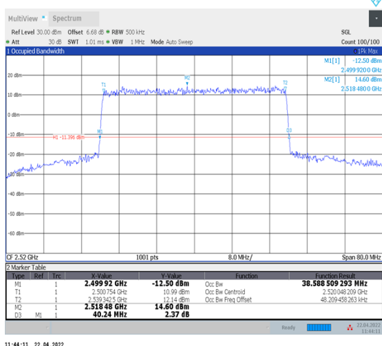
1-N7--15-40-L-1-DFT-QPSK-Outer_Full-216@0-Ant1-38.595-40.240-≤40-PASS
