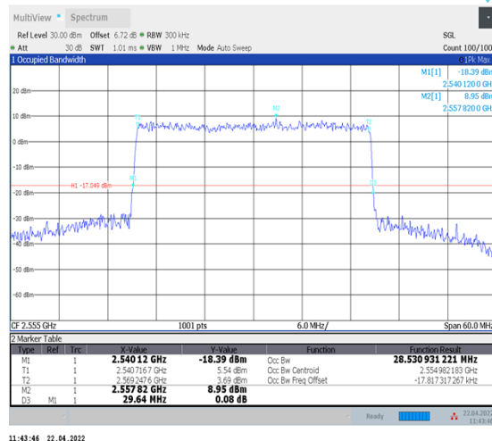
1-N7--15-30-H-9-CP-256QAM-Outer_Full-160@0-Ant1-28.533-29.640-≤30-PASS
