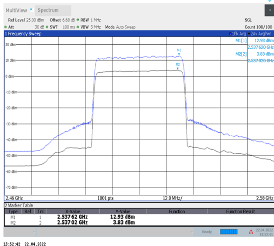
1-N7--15-40-L-1-DFT-256QAM-Outer_Full-216@0- Ant1-9.10-100%-0.00-9.10-PASS-≤13
