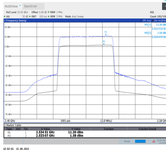
1-N7--15-40-L-2-CP-256QAM-Outer_Full-216@0- Ant1-9.72-100%-0.00-9.72-PASS-≤13
