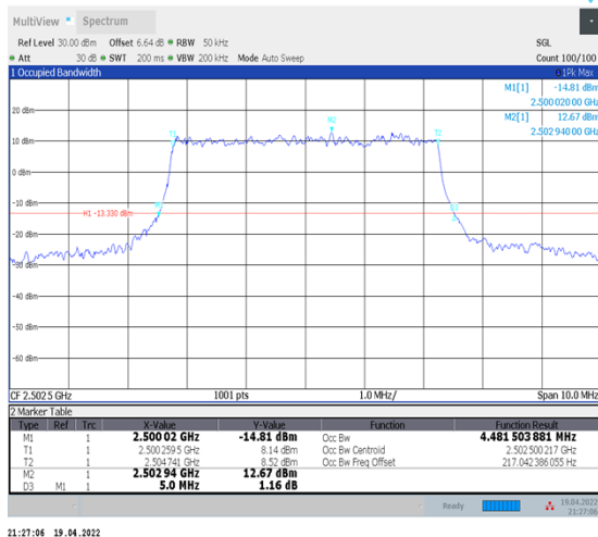
1-N7--15-5-L-3-DFT-16QAM-Outer_Full-25@0-Ant1-4.482-5.000-≤5-PASS
