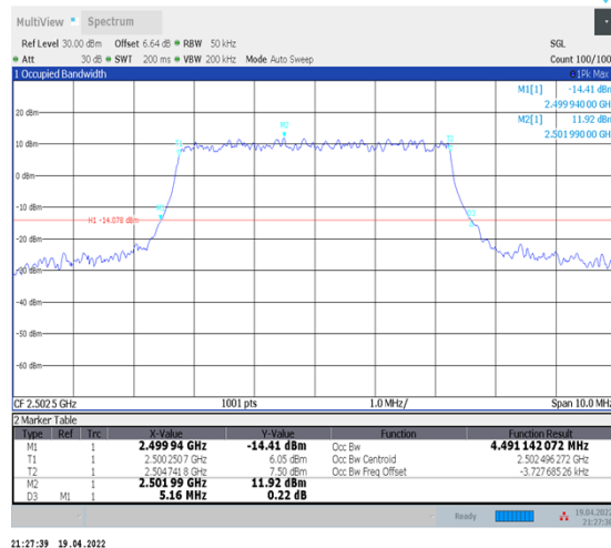
1-N7--15-5-L-4-DFT-64QAM-Outer_Full-25@0-Ant1-4.491-5.160-≤5-PASS
