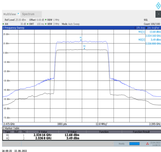
1-N7--15-40-M-1-DFT-256QAM-Outer_Full-216@0- Ant1-9.19-100%-0.00-9.19-PASS-≤13
