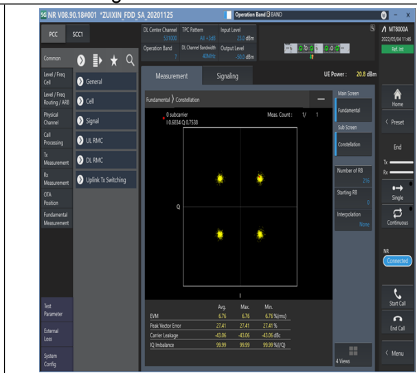
1-N7-PC3-15-40-M-6-CP-QPSK-Outer_Full-216@0-Ant1-see graph-PASS
