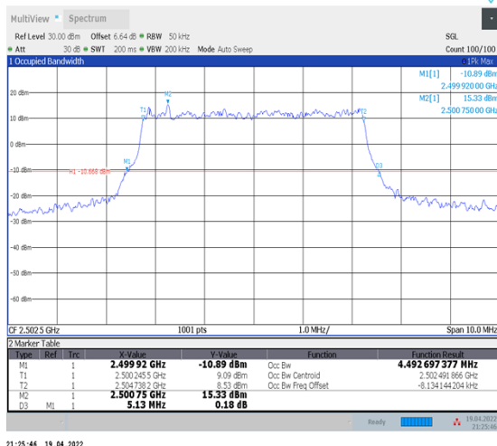
1-N7--15-5-L-1-DFT-QPSK-Outer_Full-25@0-Ant1-4.493-5.130-≤5-PASS
