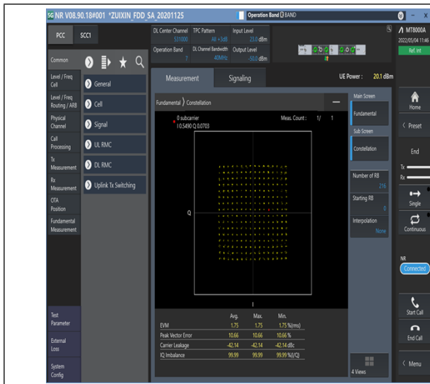
1-N7-PC3-15-40-M-5-DFT-256QAM-Outer_Full-216@0-Ant1-see graph-PASS
