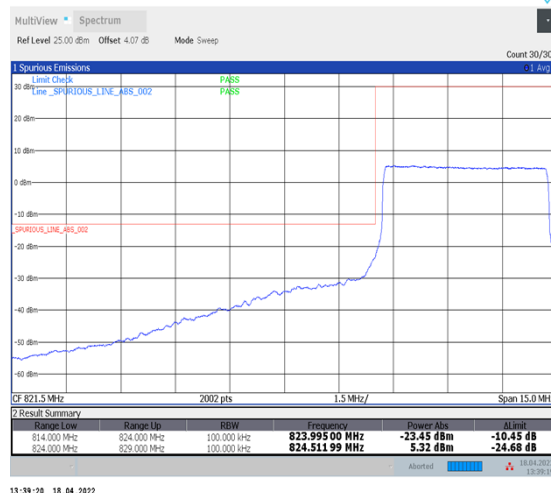
1-N5--15-5-L-6-CP-QPSK-Outer_Full-25@0-Ant1-seegraph-PASS-see graph
