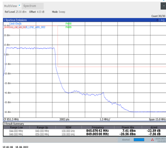
1-N5--15-5-H-3-DFT-PI2BPSK-Outer_Full-25@0-Ant1-seegraph-PASS-see graph
