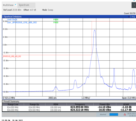
1-N5--15-5-L-4-CP-QPSK-Edge_1RB_Left-1@0-Ant1-seegraph-PASS-see graph
