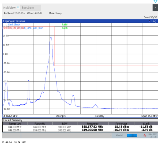
1-N5--15-5-H-5-CP-QPSK-Edge_1RB_Right-1@24-Ant1-seegraph-PASS-see graph
