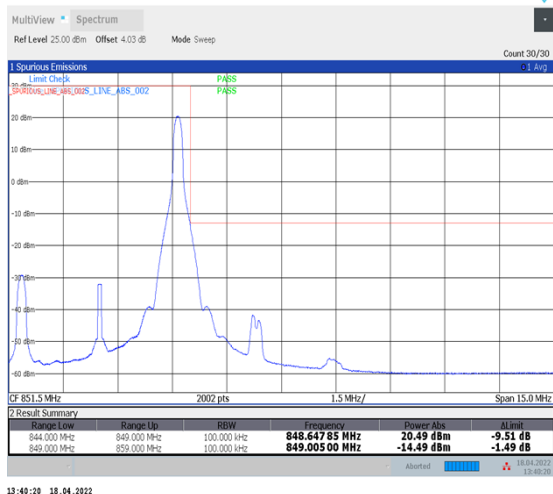
1-N5--15-5-H-2-DFT-PI2BPSK-Edge_1RB_Right-1@24-Ant1-seegraph-PASS-see graph
