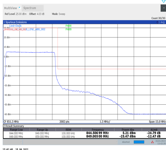
1-N5--15-5-H-6-CP-QPSK-Outer_Full-25@0-Ant1-seegraph-PASS-see graph
