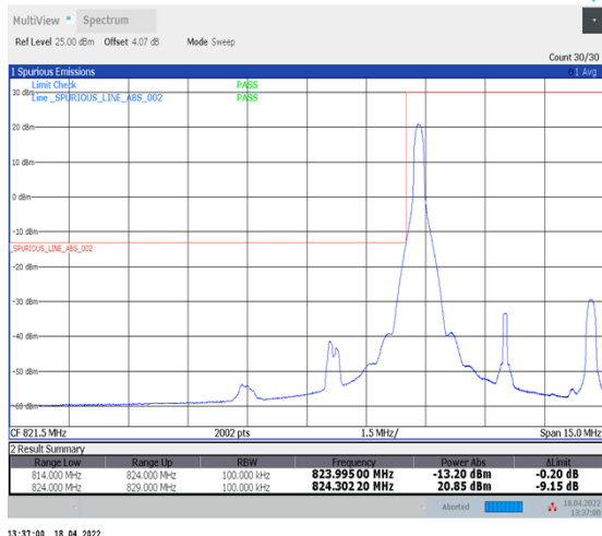
1-N5--15-5-L-1-DFT-PI2BPSK-Edge_1RB_Left-1@0-Ant1-seegraph-PASS-see graph
