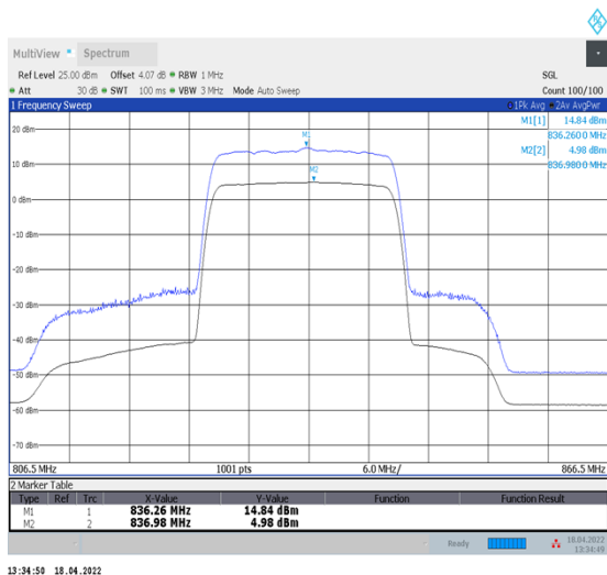
1-N5--15-20-M-1-DFT-256QAM-Outer_Full-100@0- Ant1-9.86-100%-0.00-9.86-PASS-≤13
