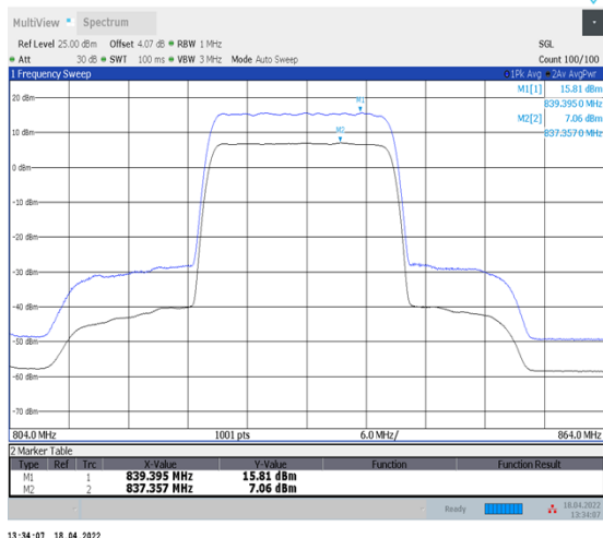
1-N5--15-20-L-1-DFT-256QAM-Outer_Full-100@0- Ant1-8.75-100%-0.00-8.75-PASS-≤13
