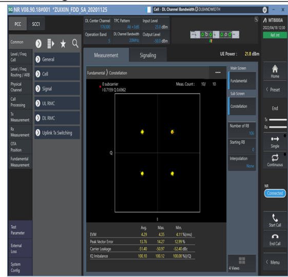
1-N5--15-20-M-6-CP-QPSK-Outer_Full-106@0-Ant1-see graph-PASS
