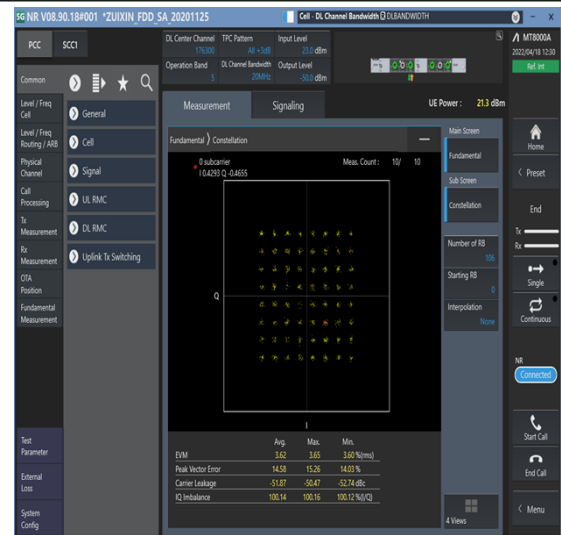
1-N5--15-20-M-8-CP-64QAM-Outer_Full-106@0-Ant1-see graph-PASS
