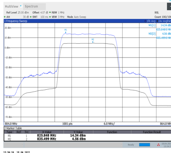
1-N5--15-20-L-2-CP-256QAM-Outer_Full-106@0- Ant1-9.78-100%-0.00-9.78-PASS-≤13
