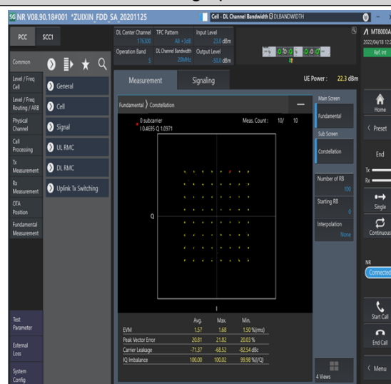
1-N5--15-20-M-4-DFT-64QAM-Outer_Full-100@0- Ant1-see graph-PASS
