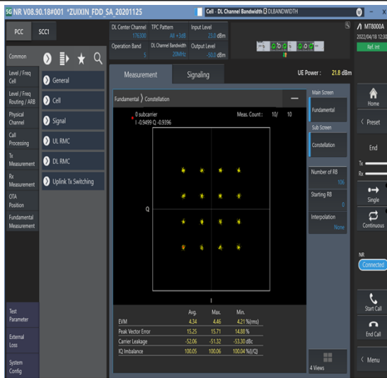
1-N5--15-20-M-7-CP-16QAM-Outer_Full-106@0-Ant1-see graph-PASS
