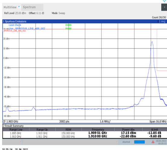
1-N2--15-15-H-5-CP-QPSK-Edge_1RB_Right-1@78-Ant1-seegraph-PASS-see graph
