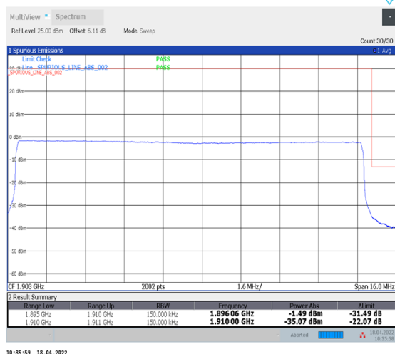
1-N2--15-15-H-6-CP-QPSK-Outer_Full-79@0-Ant1-seegraph-PASS-see graph
