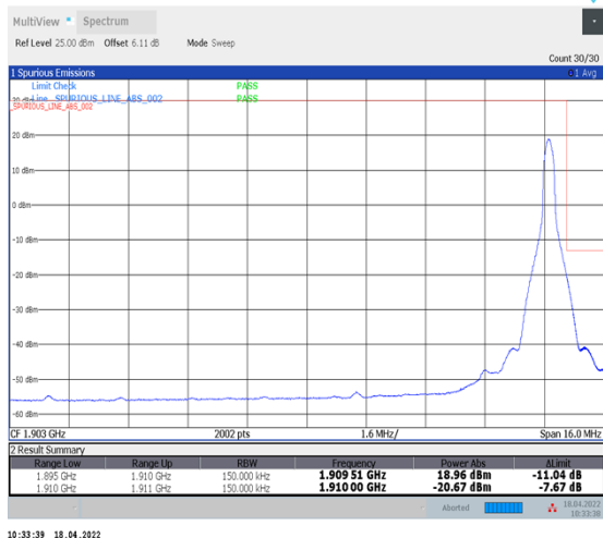
1-N2--15-15-H-2-DFT-PI2BPSK-Edge_1RB_Right-1@78-Ant1-seegraph-PASS-see graph
