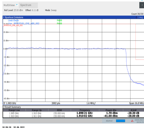
1-N2--15-15-H-3-DFT-PI2BPSK-Outer_Full-75@0-Ant1-seegraph-PASS-see graph
