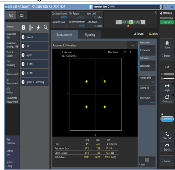
1-N2-PC3-15-20-M-6-CP-QPSK-Outer_Full-106@0-Ant1-see graph-PASS
