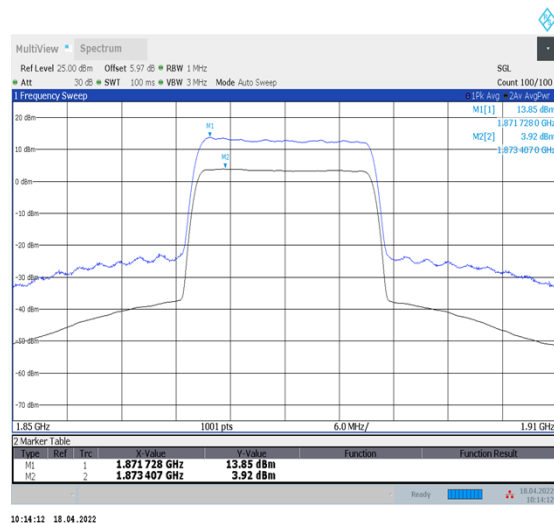
1-N2--15-20-M-2-CP-256QAM-Outer_Full-106@0- Ant1-9.93-100%-0.00-9.93-PASS≤13
