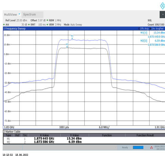
1-N2--15-20-M-1-DFT-256QAM-Outer_Full-100@0- Ant1-8.75-100%-0.00-8.75-PASS≤13
