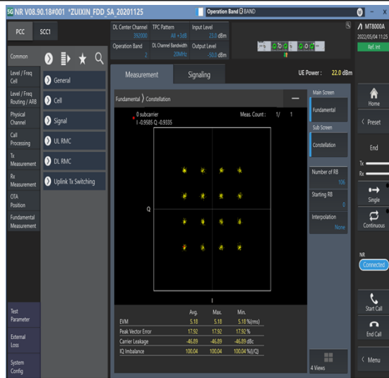
1-N2-PC3-15-20-M-7-CP-16QAM-Outer_Full-106@0-Ant1-see graph-PASS
