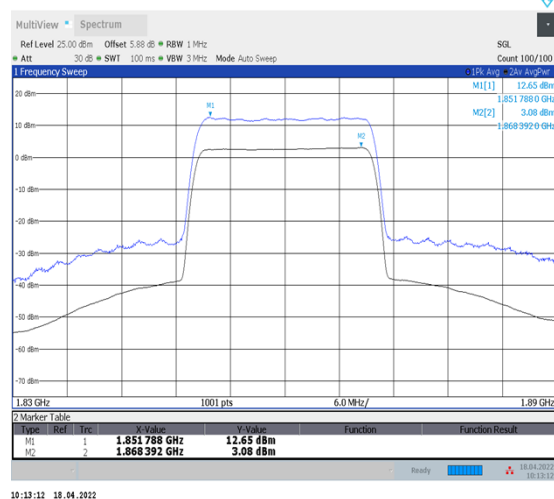
1-N2--15-20-L-2-CP-256QAM-Outer_Full-106@0- Ant1-9.57-100%-0.00-9.57-PASS≤13
