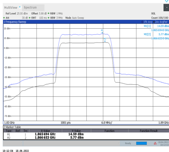
1-N2--15-20-L-1-DFT-256QAM-Outer_Full-100@0- Ant1-8.82-100%-0.00-8.82-PASS≤13
