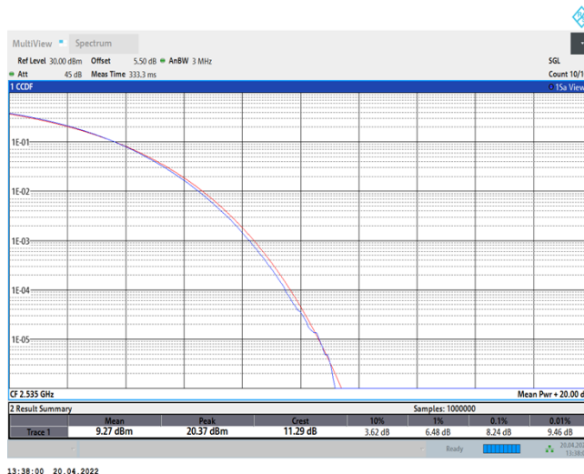
7-7-20MHz-20MHz-QPSK-QPSK-21001-21199-100RB#0-100RB#0
