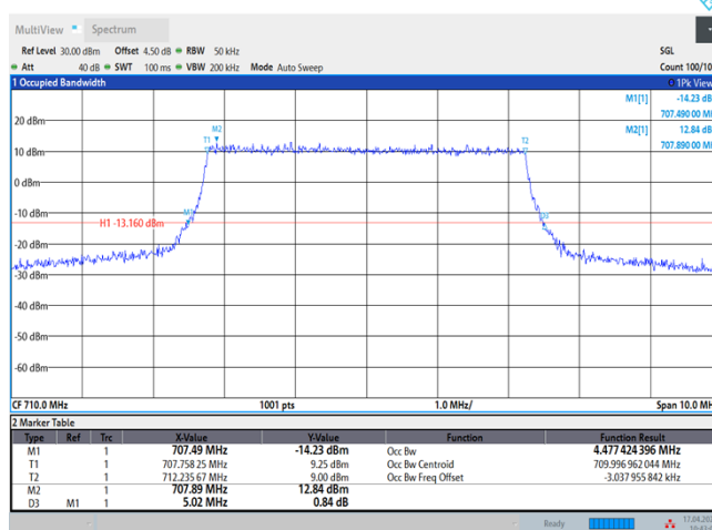
Band17-5MHz-QPSK-23790-25RB#0
