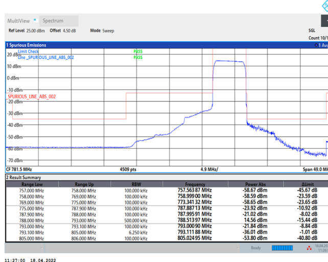
Band14-5MHz-QPSK-23305-25RB#0
