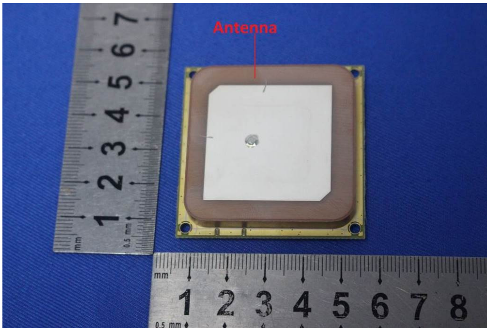
915MHz Antenna
