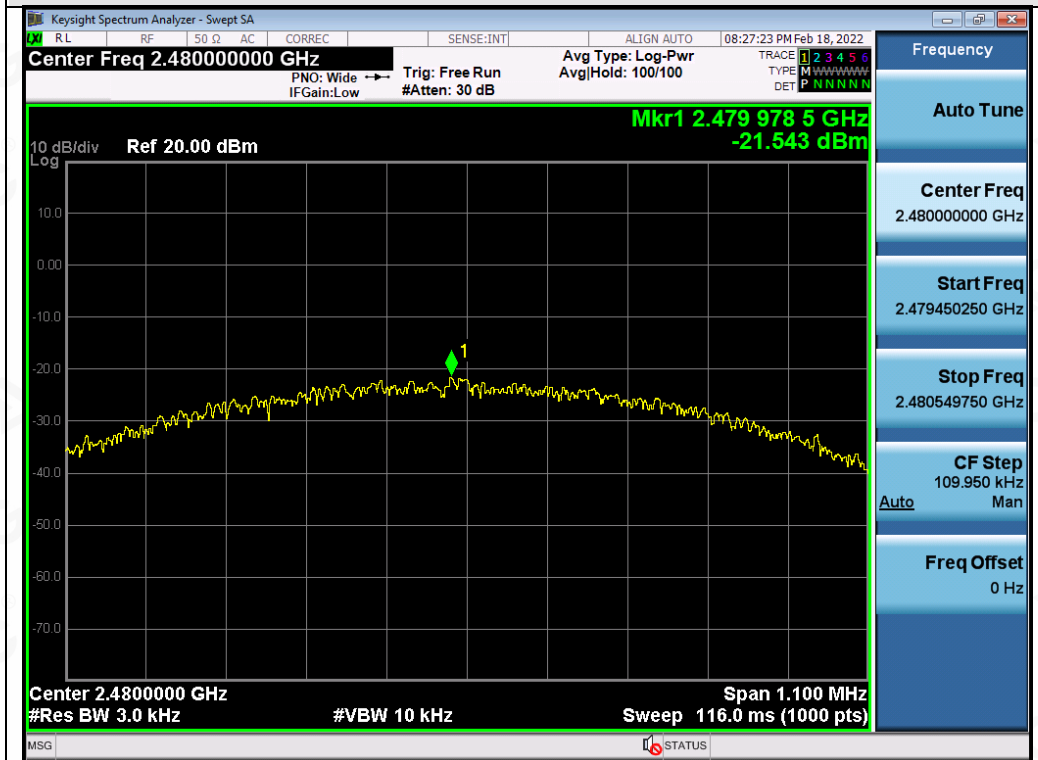
Test_Graph_LE1M_ANT1_2480_1Mbps_PSD
