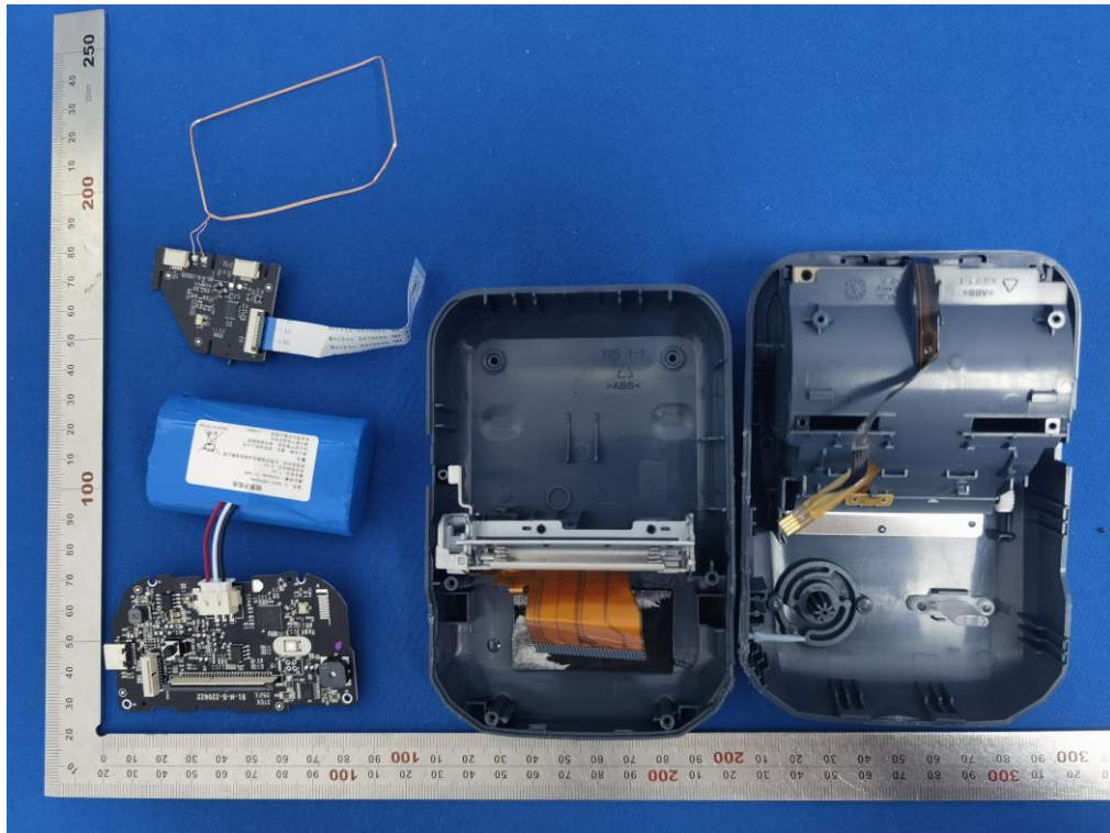
BATTERY VIEW OF EUT (JL-B201-1500mAh)
