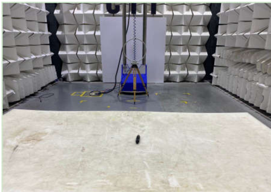
Radiated spurious emission Test Setup-1(Below 30MHz)
