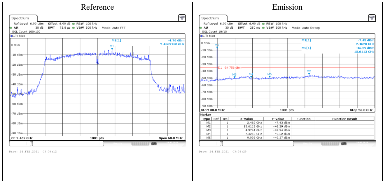
Tx. Spurious 802.11n(HT40) 2452MHz Ant1 Emission
