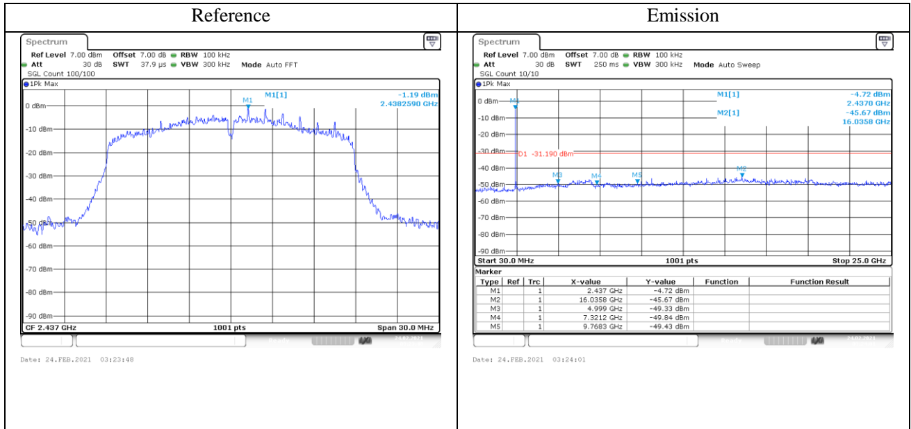
Tx. Spurious 802.11n(HT20) 2437MHz Ant1 Emission
