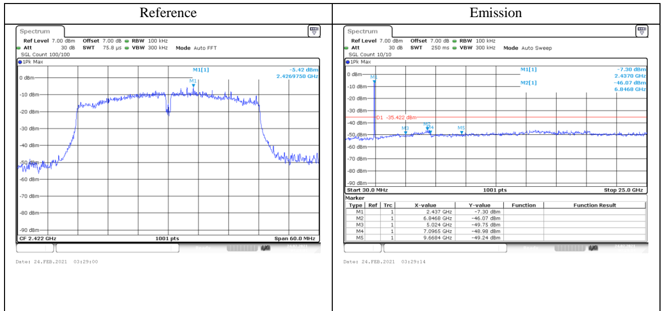
Tx. Spurious 802.11n(HT40) 2422MHz Ant1 Emission
