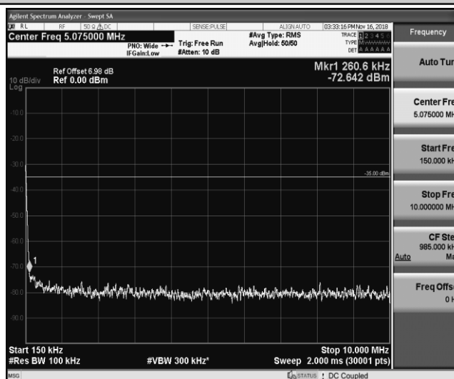
Band41_5MHz_16QAM_41315_1RB#0
