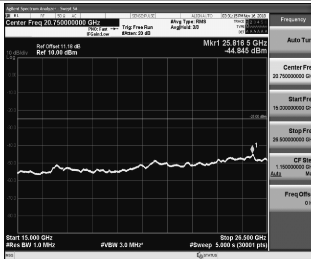
Band41_5MHz_16QAM_41315_1RB#0
