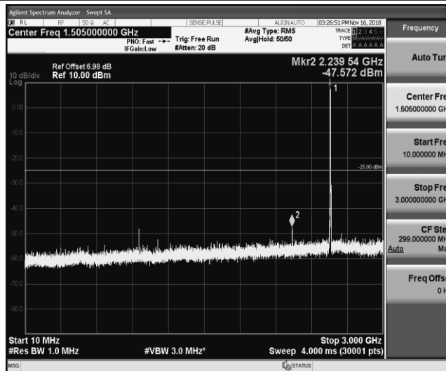
Band41_5MHz_16QAM_40265_1RB#0
