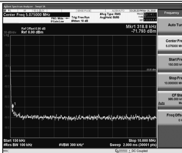
Band41_5MHz_QPSK_40620_1RB#0
