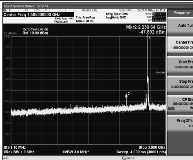
Band41_15MHz_16QAM_41165_1RB#0
