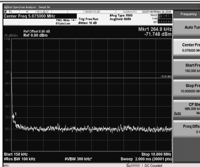
Band41_10MHz_16QAM_41190_1RB#0
