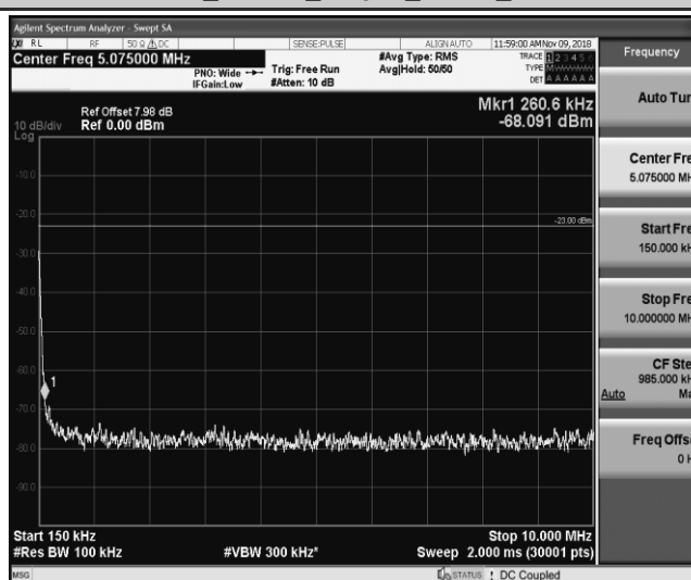
Band5_1.4MHz_16QAM_20407_1RB#0
