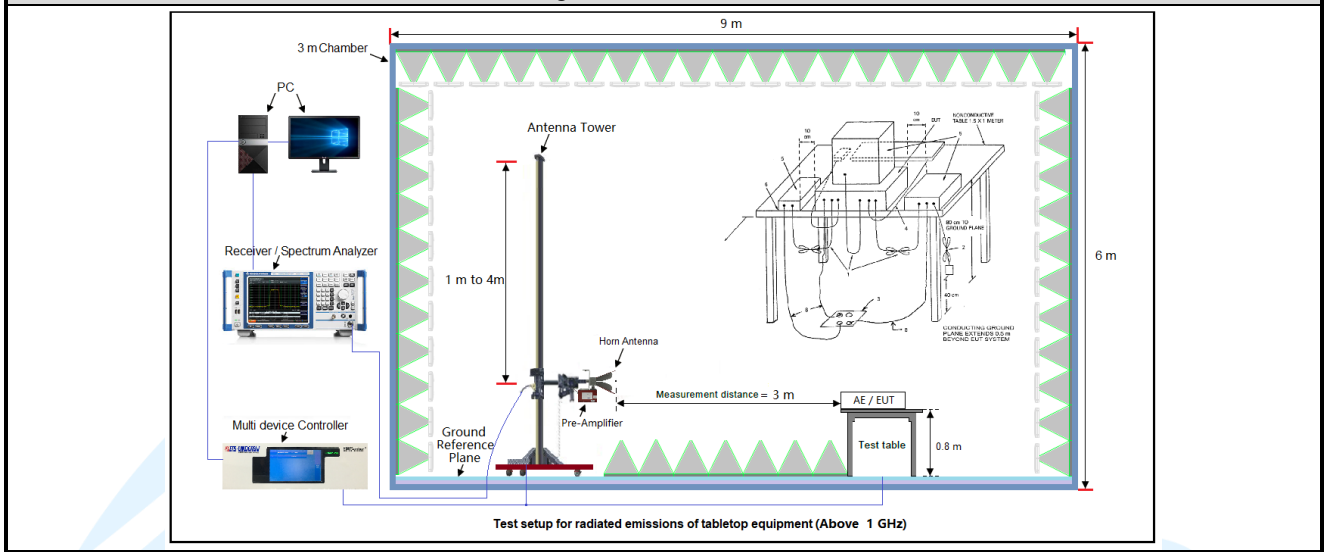
Figure 2. Above 1GHz
