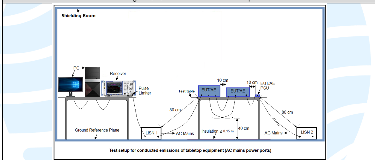
Figure 3. Conducted Emissions setup
