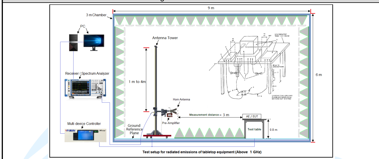
Figure 2. Above 1GHz
