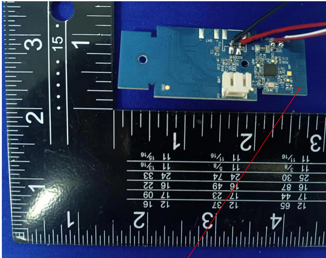
PCB antenna
