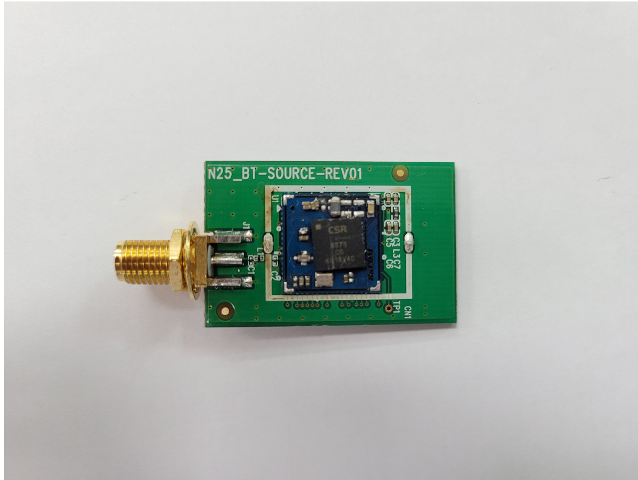
[Main board(Top)]
