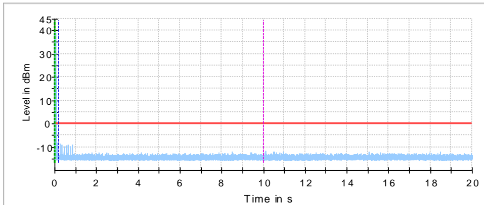
— In-Service Monitoring Channel Move Time - - - Start of Radar - - - First 200ms of Channel Closing Tx Time — Threshold - - - Trigger at end of Radar - - - 10sec Channel Move Time Limit
